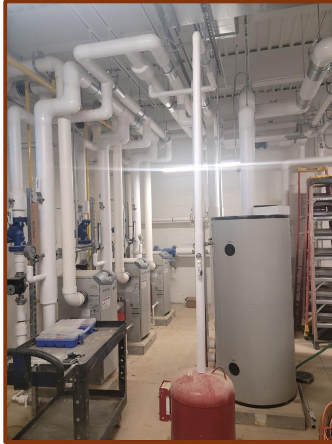
Mechanical Room – HVAC Water Heaters
