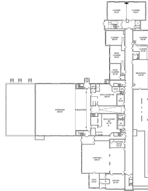
EXISTING FLOOR PLAN - BASEMENT 350' x 110' 10
