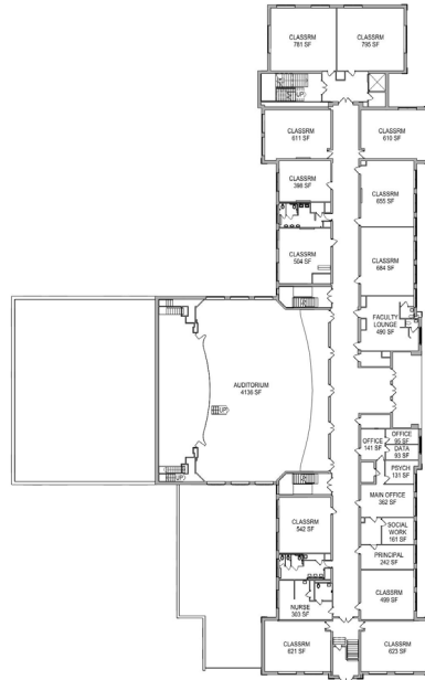
EXISTING FLOOR PLAN - FIRST FLOOR 350' x 110' 11
