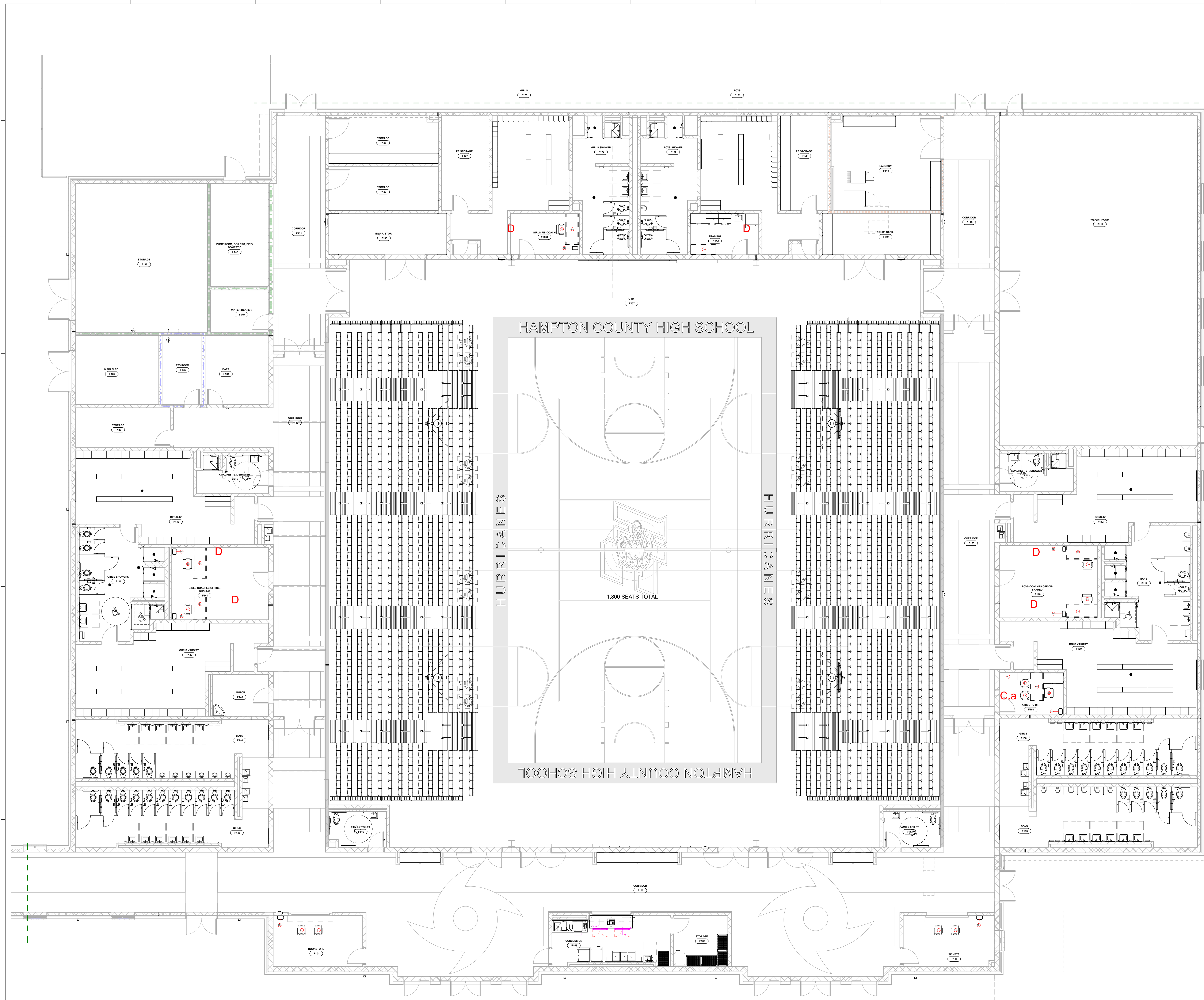
A1 FIRST FLOOR FURNITURE PLAN - BLDG F1 & F2 1/8" = 1'-0"
