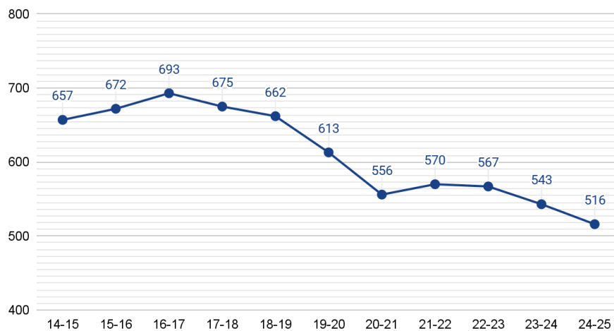
Enrollment 2014-2025
