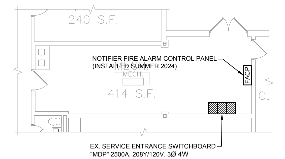
2 ELECTRICAL ROOM PLAN SCALE 1/8" = 1'-0" 0 4 8 16
