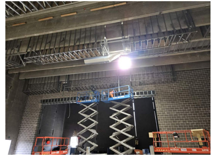
Soffit Framing at Stage Area
