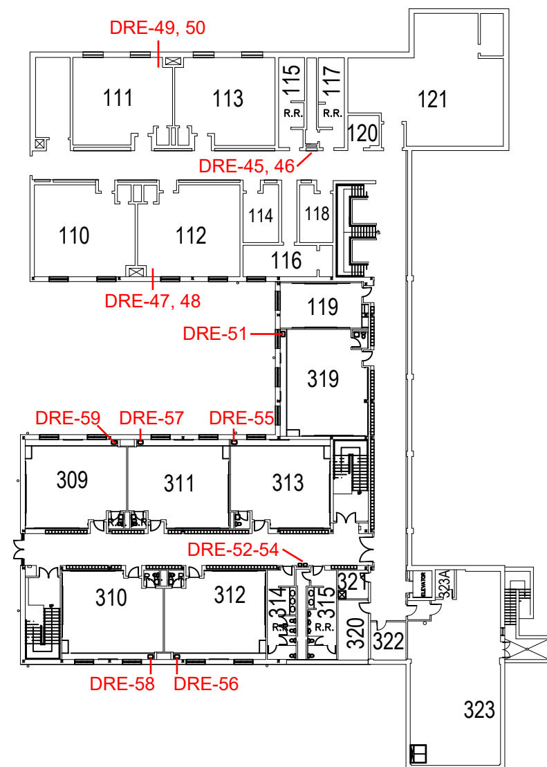
GROUND FLOOR
