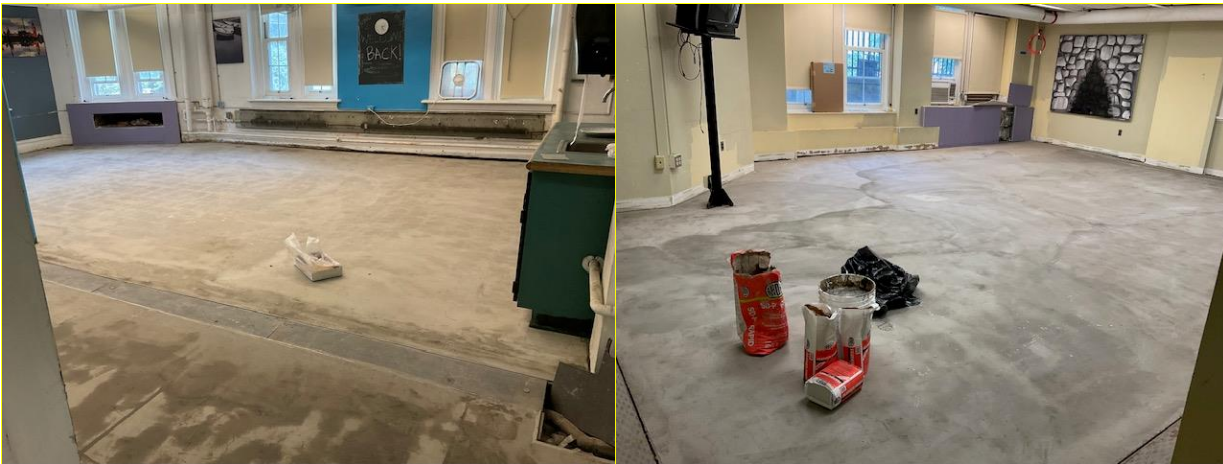
Basement- Left -: Teacher's Lounge floor prep & legacy UV openings boxed out for new UV. Right - Classroom 017 floor prep and here too legacy UV opening is boxed out for new UV. (Vinyl Tile Flooring on site. Installation expected to begin next week.)
