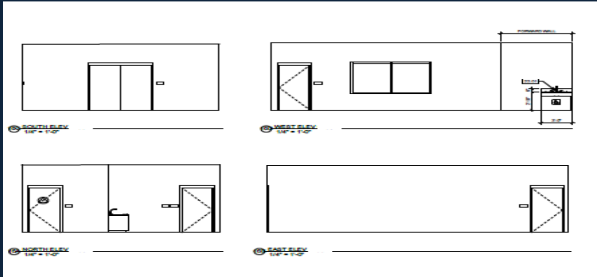
INTERIOR ELEVATIONS 16
