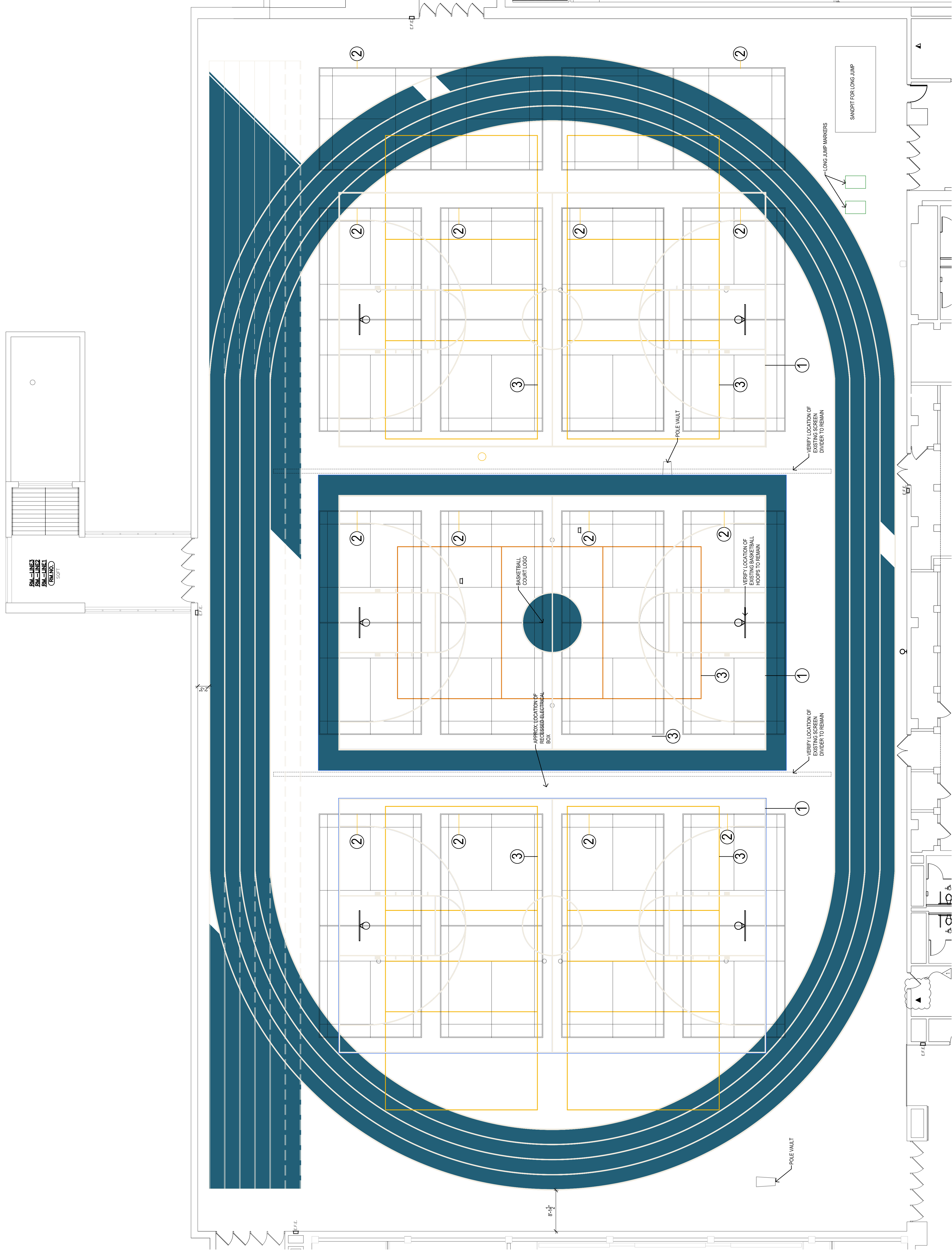
1 FLOOR PATTERN AND FINISH PLAN
