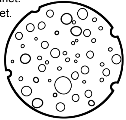
Mercury
