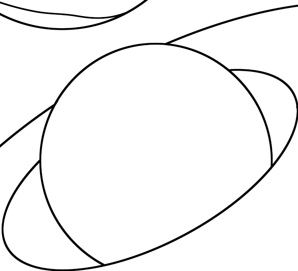
Saturn
