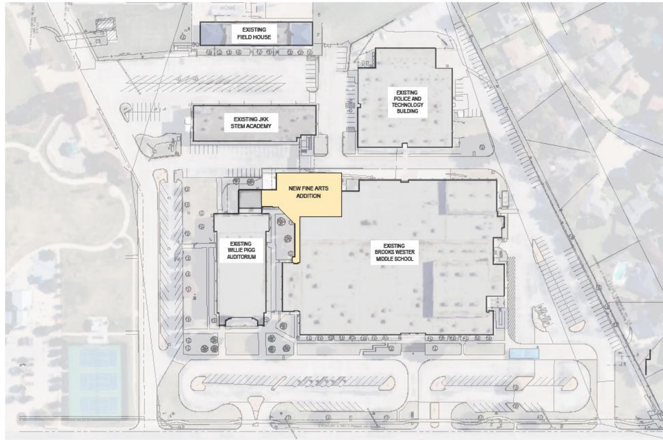
MANSFIELD I.S.D. - BROOKS WESTER MIDDLE SCHOOL - PROPOSED SITE PLAN
