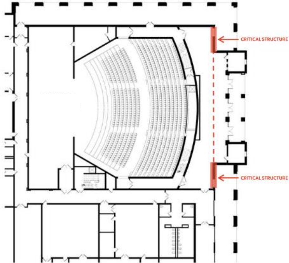
EXISTING FLOOR PLAN - LEVEL 01
