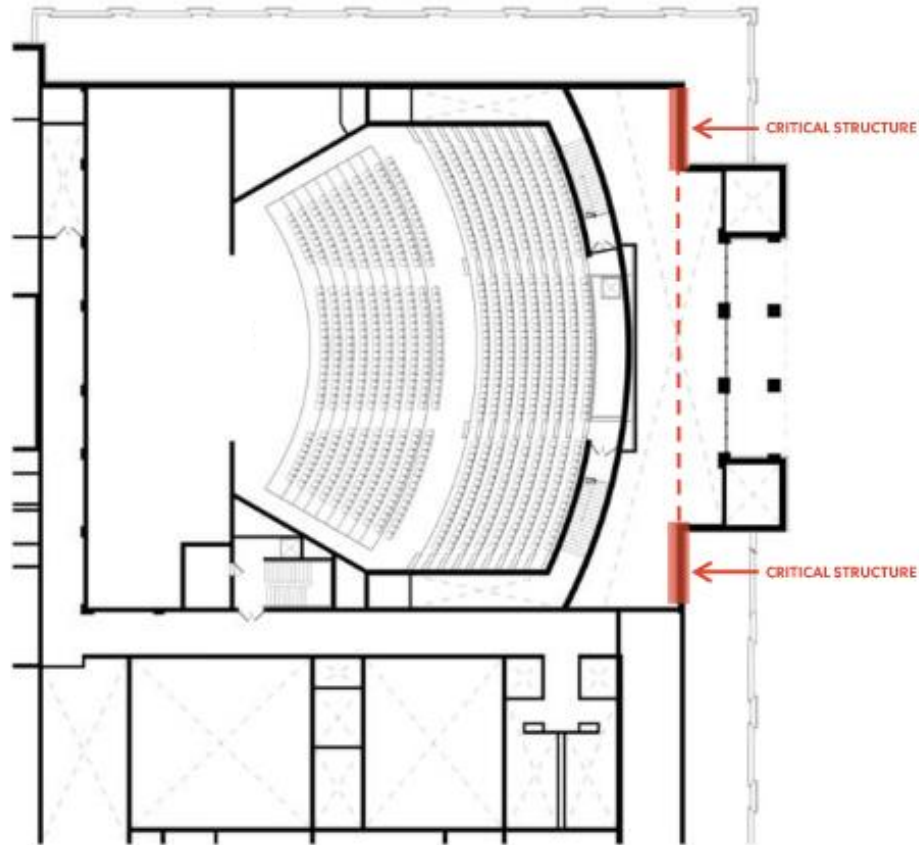
EXISTING FLOOR PLAN - LEVEL 02
