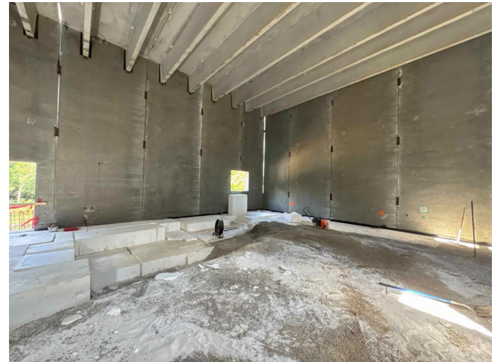
EPiC Elementary - Gym Geofoam
