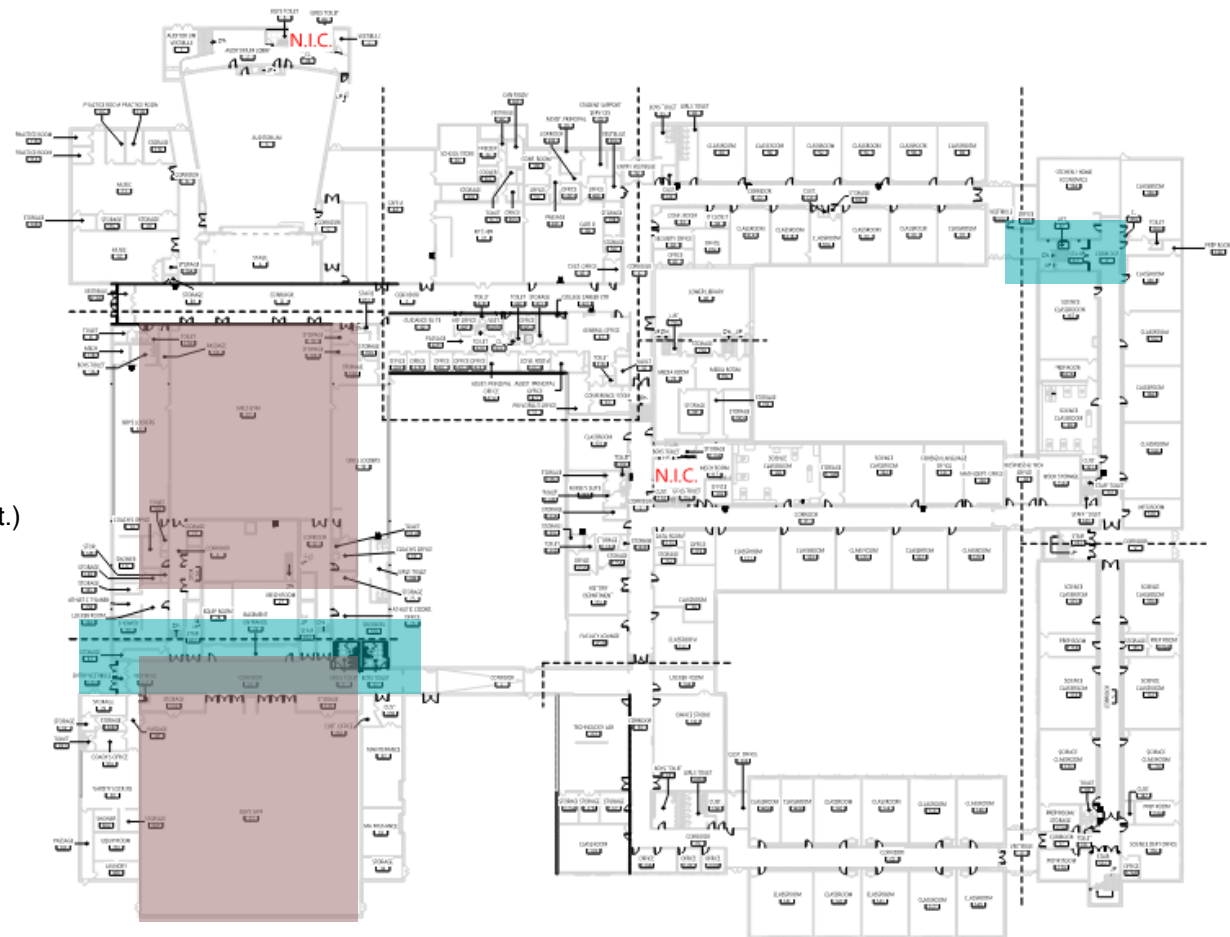
1 PHASE 1B - LOWER, MID, & GROUND FLOORS OVERALL PLAN G101-B (REV. 1-10)
