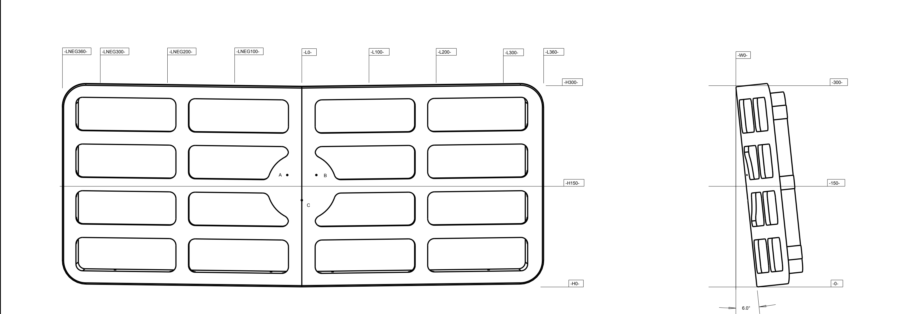
1 FRONT GRILL NOTE: BADGE PINS ATTACH TO HOLES A, B, C ON PART MATERIAL: PC ABS PLASTIC CHROMED
