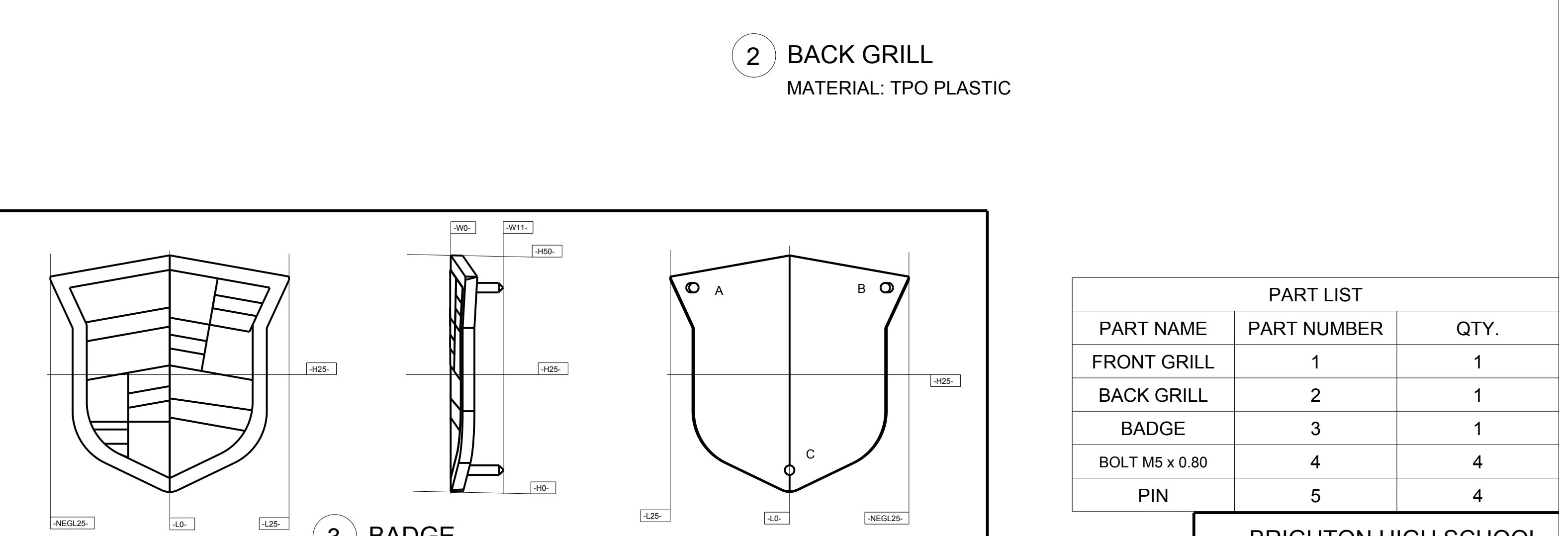
3 BADGE NOTE: BADGE ATTACHED TO PART WITH PINS A, B, C PINS OF BADGE ATTACHED WITH GLUE MATERIAL: PC ABS PLASTIC CHROMED
