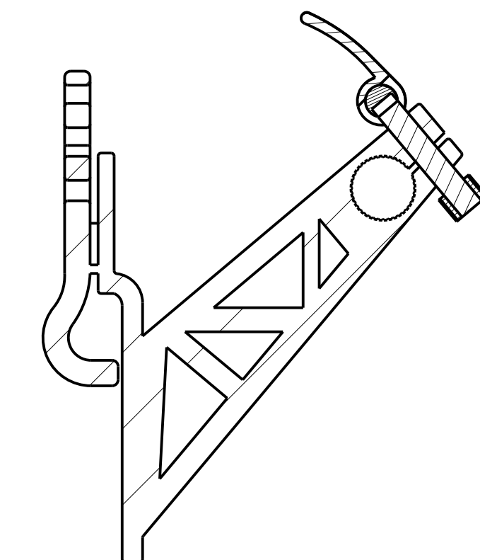
CLAMP SECTION OPEN
