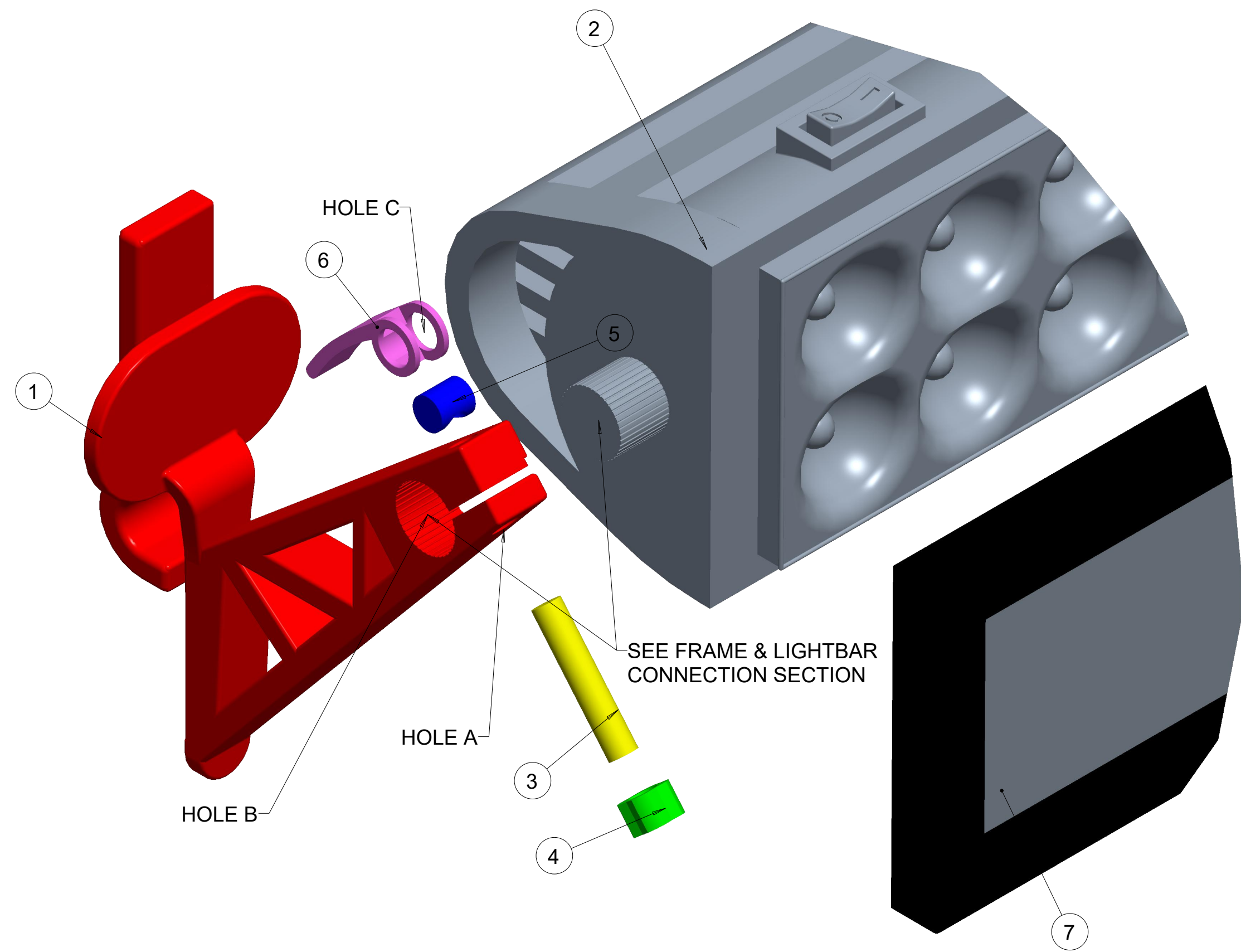
EXPLODED VIEW
