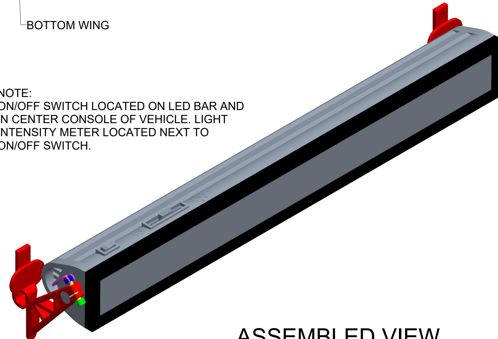
ASSEMBLED VIEW
