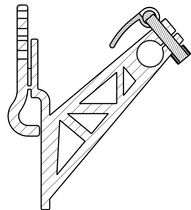
CLAMP SECTION CLOSED
