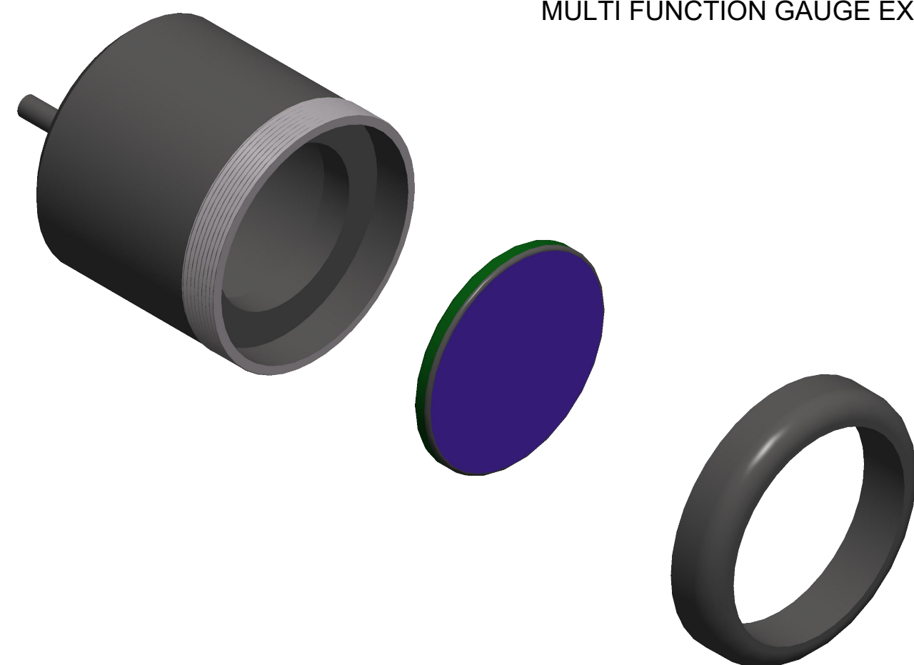
MULTI FUNCTION GAUGE EXPLODED
