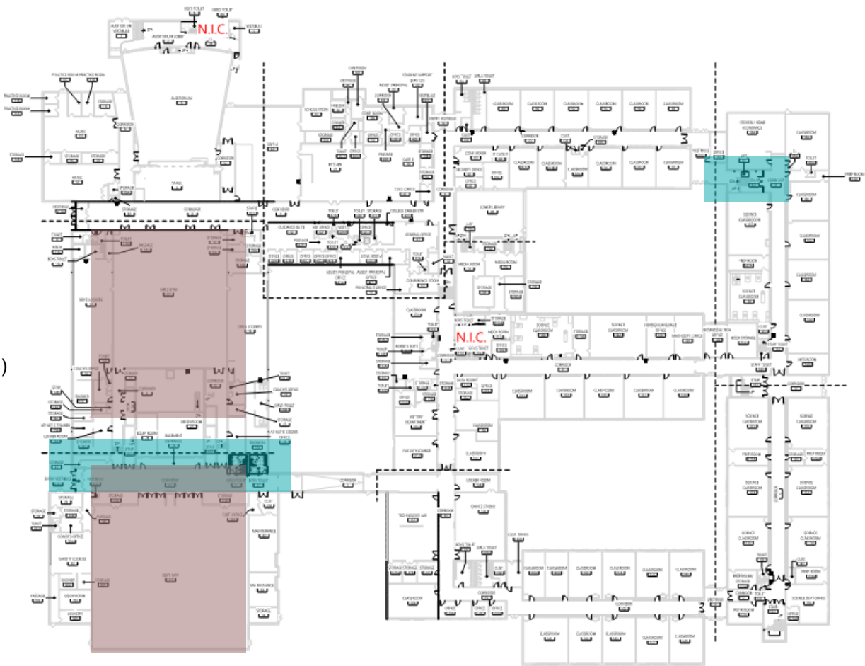
1 PHASE 1B - LOWER, MID, & GROUND FLOORS OVERALL PLAN G101-B 10/1/20
