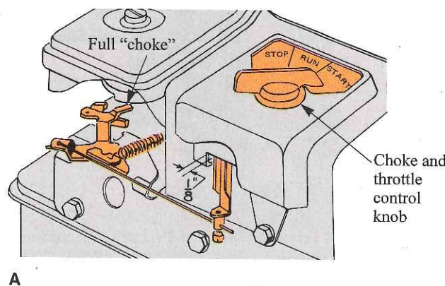
Figure 8-33. Combined manual throttle and choke control. A—The control knob turned to Start activates the choke. B—The knob turned to Stop closes the stop switch.
