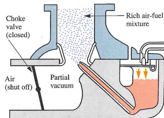
Figure 8-14. The choke valve is closed and vacuum is high in the carburetor. The fuel mixture entering the intake manifold is extremely rich.
