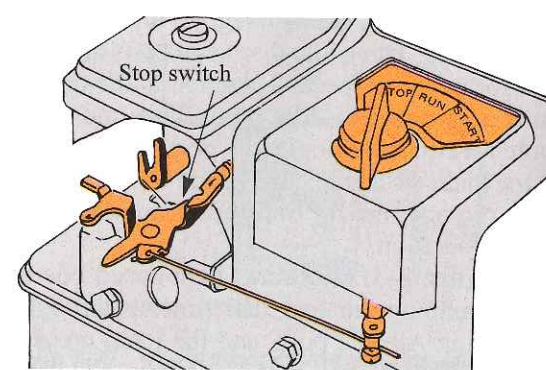
Figure 8-33. Combined manual throttle and choke control. A—The control knob turned to Start activates the choke. B—The knob turned to Stop closes the stop switch.
