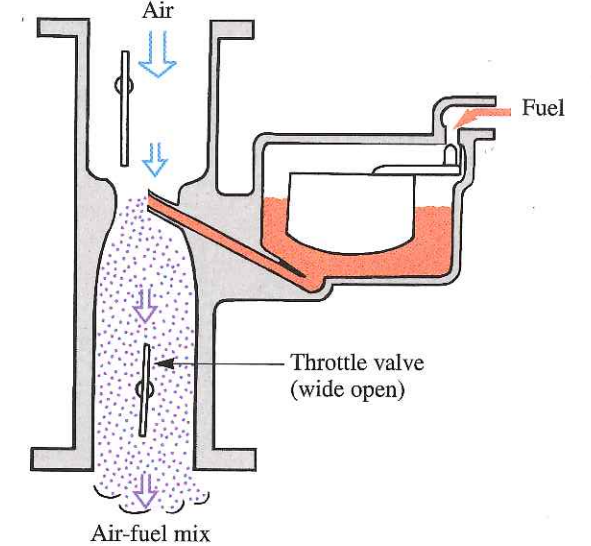
Figure 8-5. Air flowing through the venturi has reduced the pressure around the nozzle. Fuel is drawn up the nozzle by vacuum and mixes in the airstream. (Deere & Co.)
