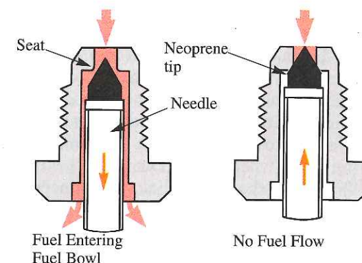
Figure 8-13. The needle in a float bowl opens and closes the fuel passage into chamber. The needle is operated by the hinged arm of the float. (Evinrude Motors)
