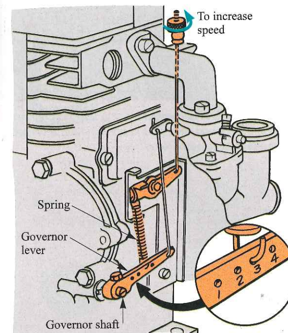
Figure 8-42. A single speed arrangement, using a knurled nut to provide a limited governor speed range. (Briggs and Stratton Corp.)
