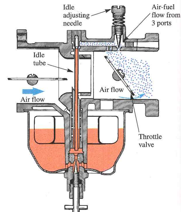
Figure 8-22. Part throttle. The engine is running from the primary and secondary orifices.
