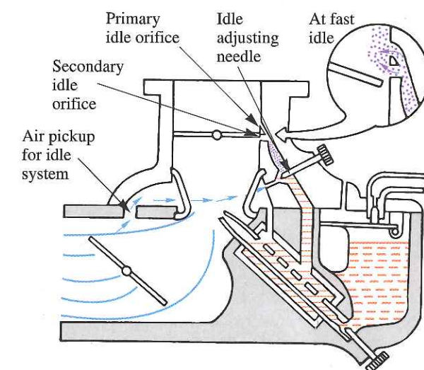
Figure 8-19. During idling, some incoming air is directed through a passage around the venturi. This air mixes with fuel and is drawn out the primary and secondary idle orifices. The throttle valve is closed for idle and slightly opened for fast idle.
