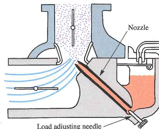
Figure 8-16. A load adjusting needle, located as shown, regulates the amount of fuel entering the main nozzle.
