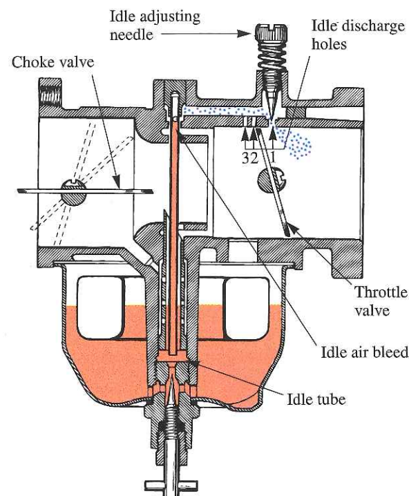
Figure 8-21. Idling. The throttle valve is closed, and the engine is operating from the primary idle orifice. (Zenith Div., Bendix Corp.)
