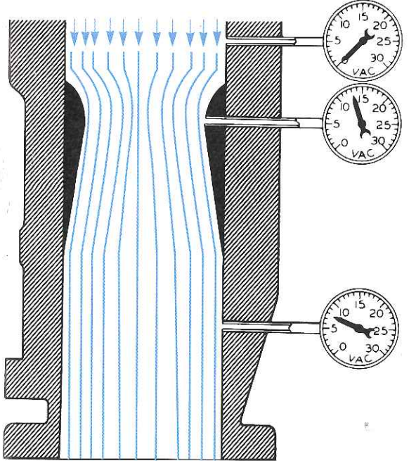
Figure 8-4. The venturi principle. A restriction in a passage causes incoming air to increase its velocity, while pressure is reduced. Reduction in pressure draws fuel into the airstream.
