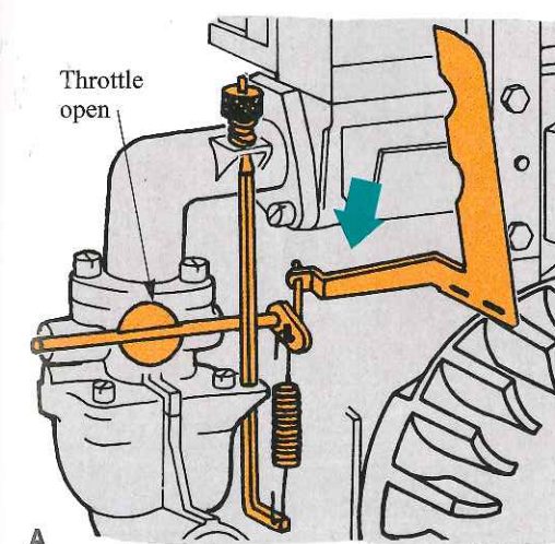
Figure 8-39. Air vane governor. A—With the engine stopped, the spring holds the throttle open. B—With the engine running, air pressure pivots the vane of the fixed-speed governor and shuts the throttle valve until the spring pressure and the vane pressure are balanced. A knurled nut alters the spring tension and adjusts the speed. (Briggs and Stratton Corp.)
