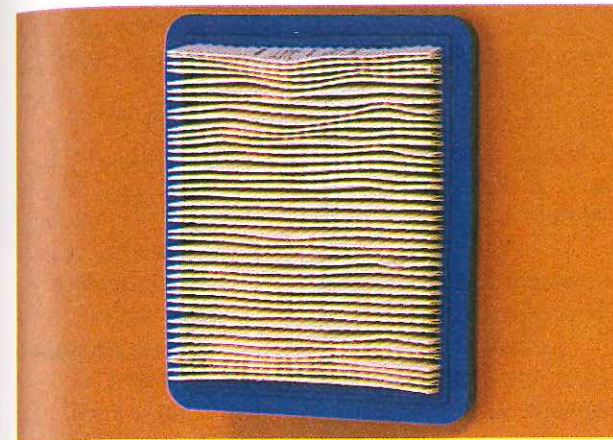
Figure 8-52. Air and dust particles travel through the pleated paper filter element, trapping dust. Clean air continues to the engine. A gasket seals the element.
