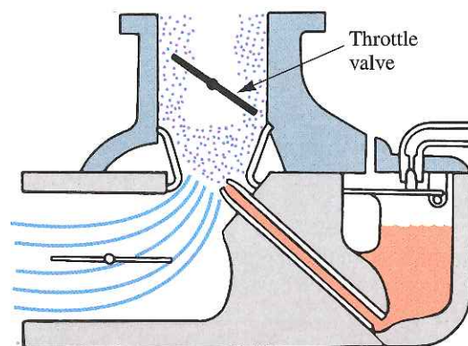
Figure 8-15. The throttle valve is located downstream from the main fuel nozzle. The throttle regulates the amount of air-fuel mixture entering the engine.
