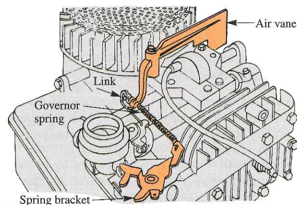
Figure 8-40. A variable speed air vane governor. To change rpm, the operator alters the governor spring tension by rotating the spring bracket.
