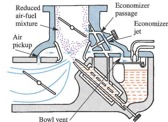
Figure 8-18. An economizer system creates a reduced pressure in the float bowl during part-throttle operation, which retards the amount of fuel discharged from the main nozzle.
