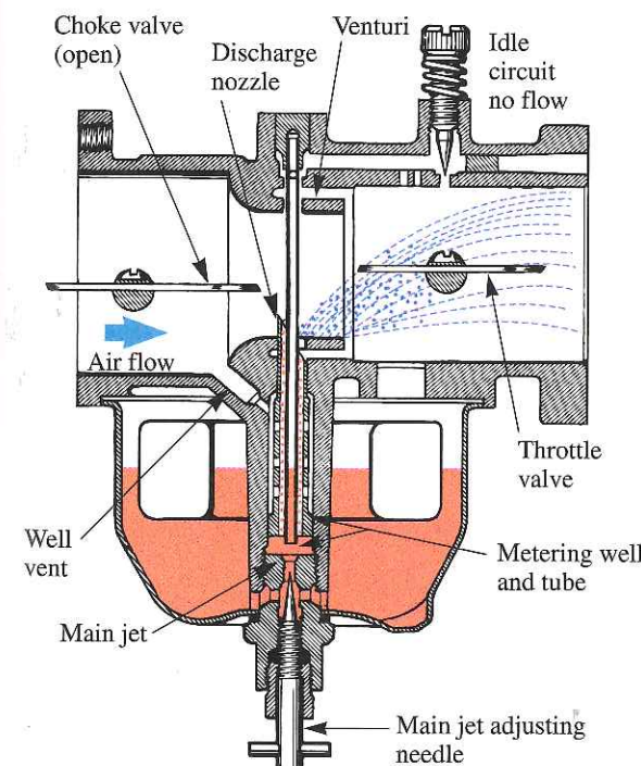
Figure 8-23. Full throttle. The idle orifices have stopped feeding fuel due to the reduced vacuum in that part of the carburetor. A full flow of fuel is being drawn from the main nozzle.
