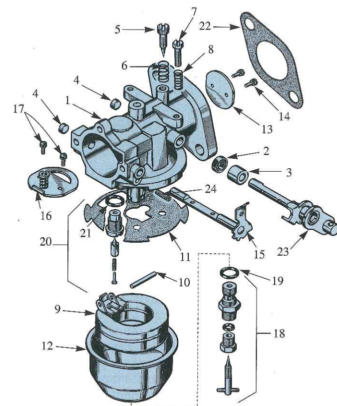
Figure 8-24. An exploded view of a natural draft carburetor: 1—Throttle body. 2—Seal. 3—Retainer. 4—Cup rings. 5—Idle adjustment needle. 6—Spring. 7—Throttle stop screw. 8—Spring. 9—Float and hinge assembly. 10—Float pin. 11—Gasket. 12—Fuel bowl. 13—Throttle valve. 14—Screw. 15—Lever and shaft assembly for choke. 16—Choke valve. 17—Screw. 18—Main jet and adjustment assembly. 19—Washer. 20—Fuel valve and seat assembly. 21—Gasket. 22—Flange gasket. 23—Throttle shaft and lever assembly. 24—Spring. (Zenith Div., Bendix Corp.)
