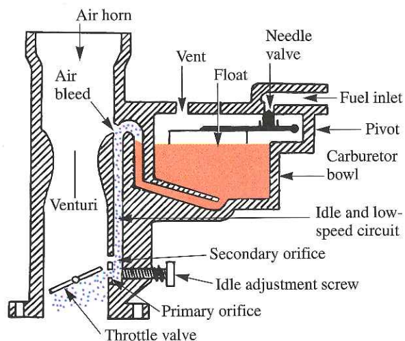
Figure 8-20. In a downdraft carburetor, the incoming air enters in the air bleed above the venturi and travels with fuel to the idle orifice. The carburetor is in an idling state, since the throttle valve has uncovered the primary orifice only. (Deere & Co.)
