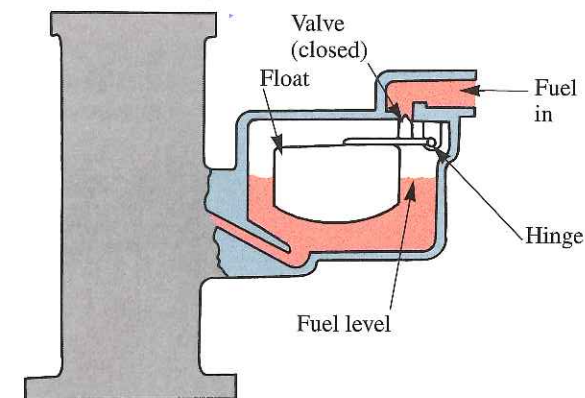
Figure 8-12. The float in a float bowl maintains a constant fuel level. When the fuel level rises, the float closes the needle valve, stopping incoming fuel. When the fuel level lowers, the float unseats the needle and lets more fuel in. (Deere & Co.)
