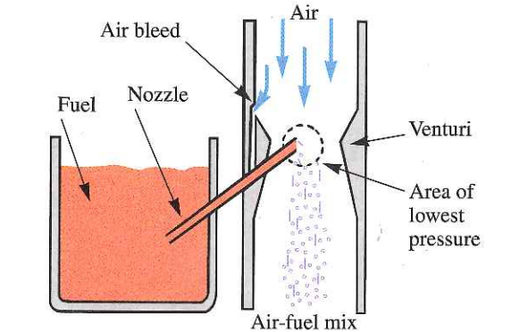
Figure 8-6. To atomize fuel into finer particles, an air bleed is used. Higher pressure of air horn forces some air to enter at a port midway in the nozzle, so fuel is partly atomized before leaving the nozzle.
