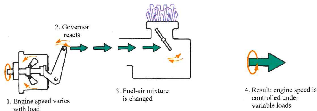
Figure 8-35. A centrifugal governor controls engine speed by the varying fuel mixture. (Deere & Co.)
