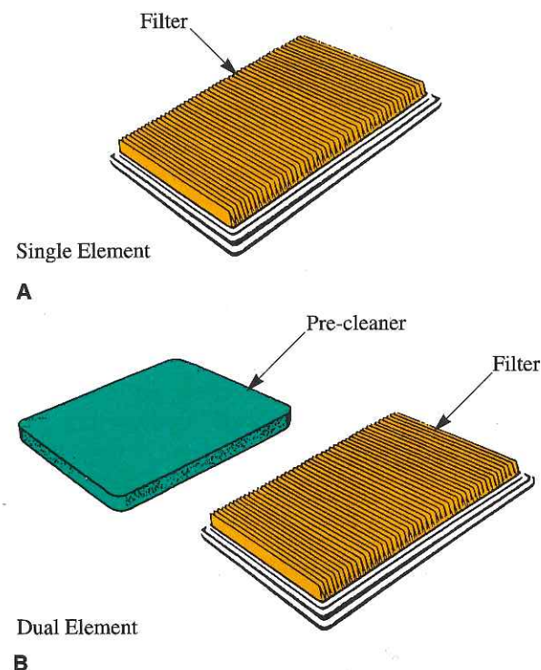
Figure 8-54. Single filters (A) are used for mild conditions. Dual-element filters (B) are used for extremely dirty conditions.
