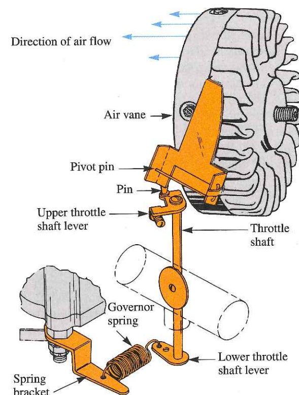
Figure 8-36. This schematic illustrates the operation of an air vane governor. The air vane tries to close the throttle valve, while the governor spring tries to open it. The balance between these two forces determines the throttle position. (Tecumseh Products Co.)
