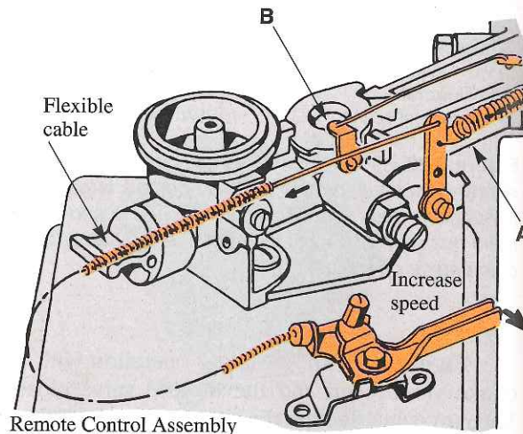
Figure 8-32. This manual throttle control uses a flexible cable to transmit motion from the hand lever to the governor spring lever. (Briggs and Stratton Corp.)
