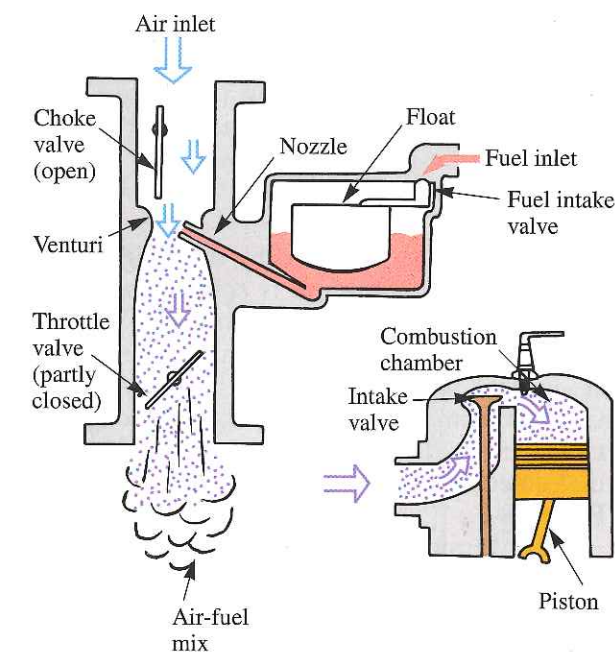
Figure 8-1. Air entering the carburetor mixes with fuel in proper proportion, and the mixture flows into the combustion chamber. (Deere & Co.)
