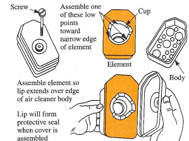
Figure 8-49. Removal of the air cleaner is relatively easy so servicing can be done regularly. (Briggs and Stratton Corp.)
