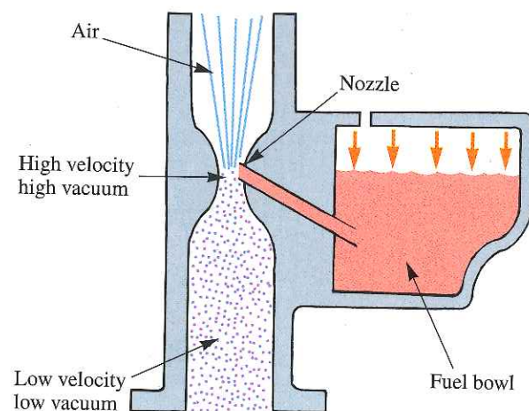
Figure 8-10. A downdraft carburetor has a downward flow of air through the venturi. Since it can operate with lower velocities, it has larger passages.
