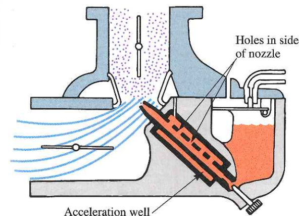
Figure 8-17. An acceleration well stores fuel for use during rapid acceleration. When the fuel has been used from the acceleration well, the nozzle holes act as air bleeds. (Deere & Co.)
