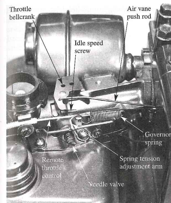
Figure 8-37. The parts of a typical governor system for an actual engine. Note the location of the idle speed screw and needle valve screw.
