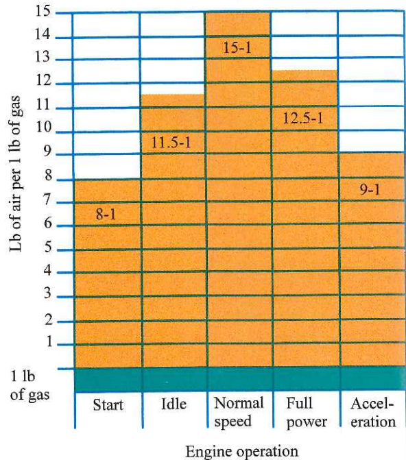
Figure 8-2. Air-fuel mixture requirements vary depending on operating conditions. This chart shows the approximate air-fuel ratios for various operating conditions.
