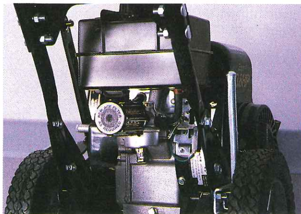
Figure 8-51. A dry-type filter element can be partially cleaned by tapping it gently. A new element should be installed as needed.
