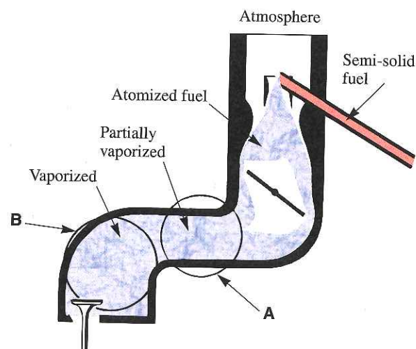
Figure 8-7. In addition to atomization caused by the air bleed and venturi, fuel is further vaporized: A—by vacuum in manifold. B—by engine heat.
