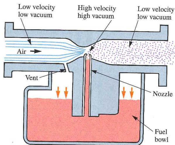
Figure 8-8. A natural draft carburetor has a horizontal air flow through it. (Deere & Co.)
