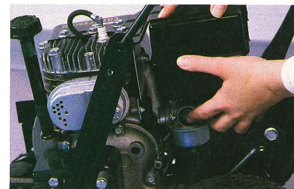
Figure 8-25. A primer plunger mounted on the carburetor.
