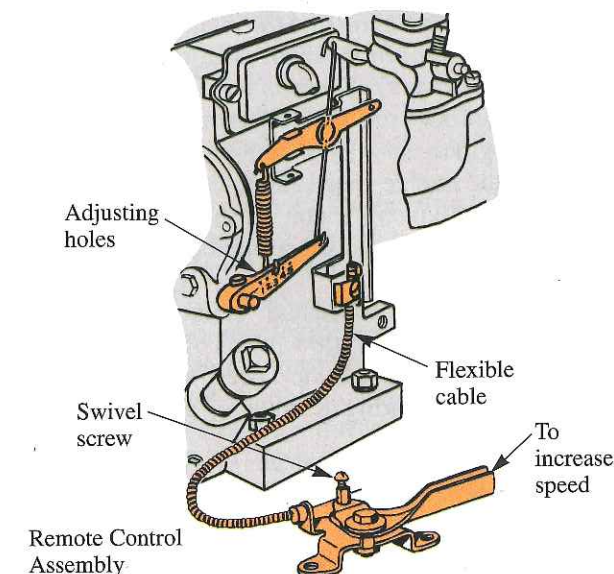
Figure 8-43. An operator-controlled governor speed setting device allows quick, wide, governed speed changes. (Briggs and Stratton Corp.)
