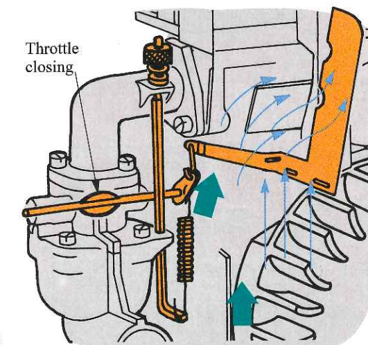
Figure 8-39. Air vane governor. A—With the engine stopped, the spring holds the throttle open. B—With the engine running, air pressure pivots the vane of the fixed-speed governor and shuts the throttle valve until the spring pressure and the vane pressure are balanced. A knurled nut alters the spring tension and adjusts the speed. (Briggs and Stratton Corp.)
