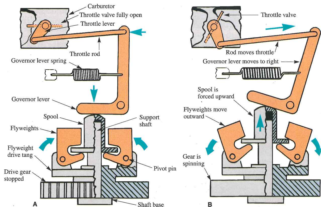
Figure 8-41. A centrifugal-type governor. Centrifugal force causes the flyweights to pivot outward, raising the spool. The spool rotates the governor lever, which closes the throttle valve. The balance between centrifugal force and governor spring tension determines the throttle valve setting.
