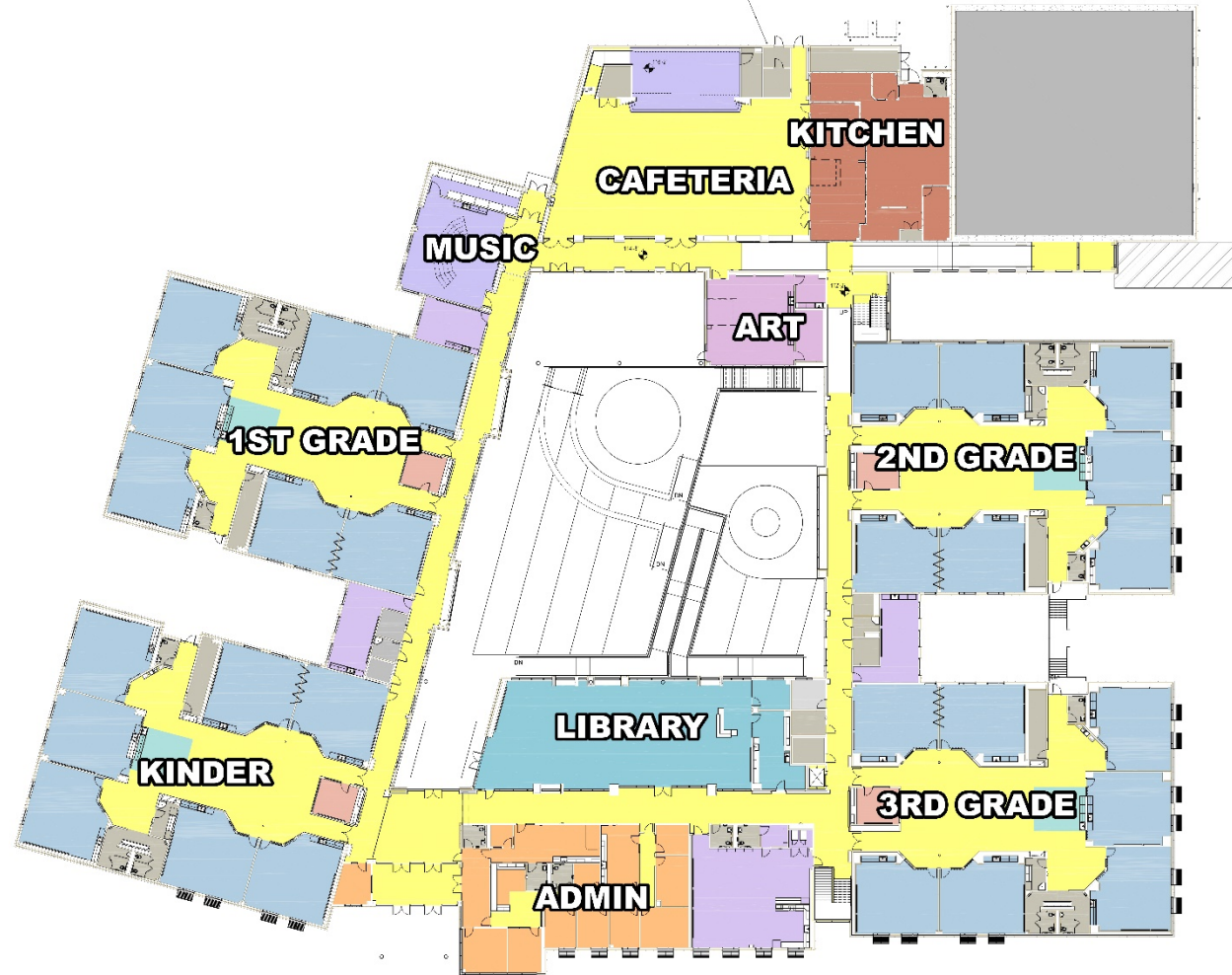
Composite First Level – Floor Plan
