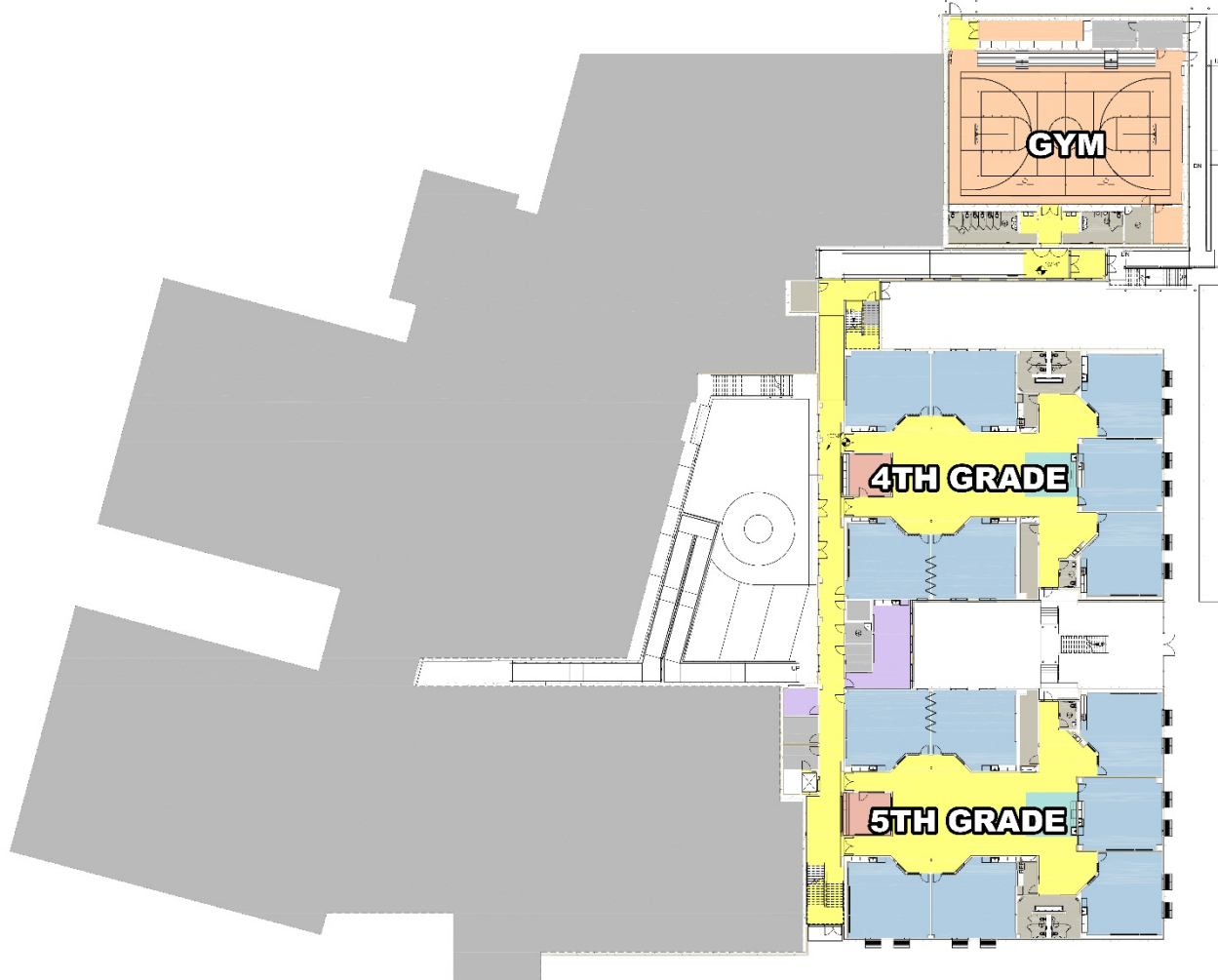
Composite Ground Level – Floor Plan
