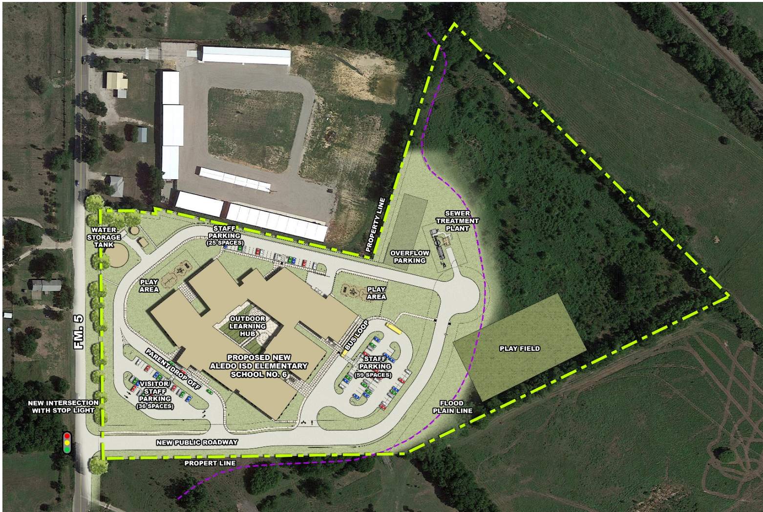
Overall Composite Site Plan
