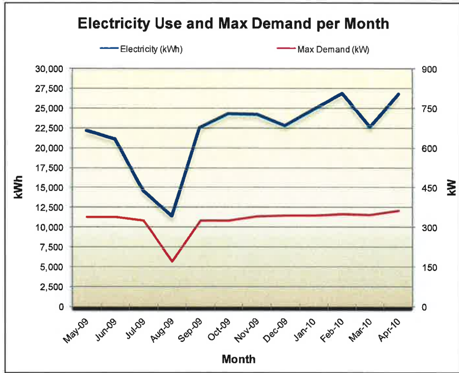
Figure 1a.Mt. Caesar Elementary School Monthly Electricity Use & Max Demand
