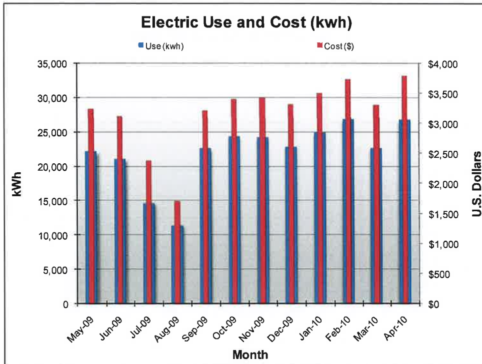
Figure 1b.Mt. Caesar Elementary School Monthly Electricity Use Vs. Cost
