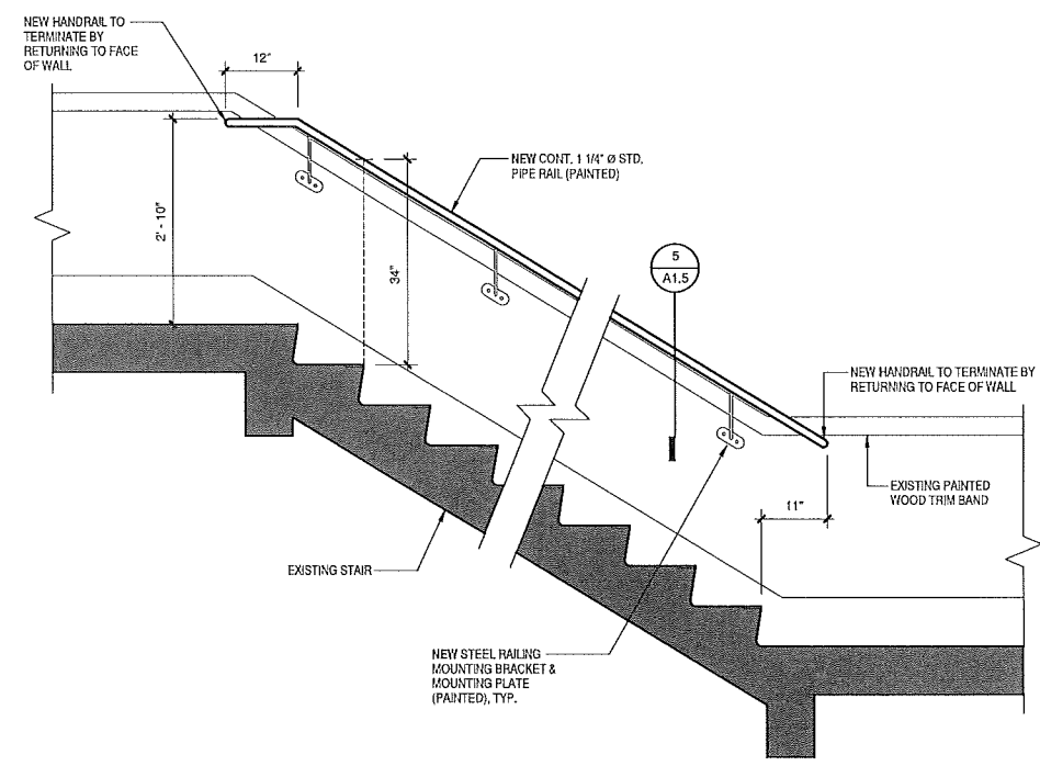
4 WALL MOUNTED RAILING ELEVATION A1.5 3/4" = 1'-0"
