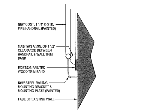
5 WALL MOUNT HANDRAIL DETAIL A1.5 1 1/2" = 1'-0"
