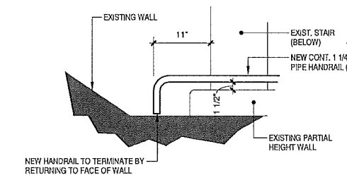
2 HANDRAIL EXTENSION A1.5 1" = 1'-0"
