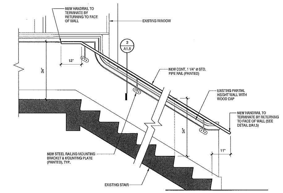
1 WALL MOUNTED RAILING ELEVATION - AT WOOD CAP A1.5 3/4" = 1'-0"
