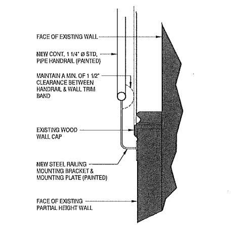
3 WALL MOUNT HANDRAIL DETAIL A1.5 1 1/2" = 1'-0"
