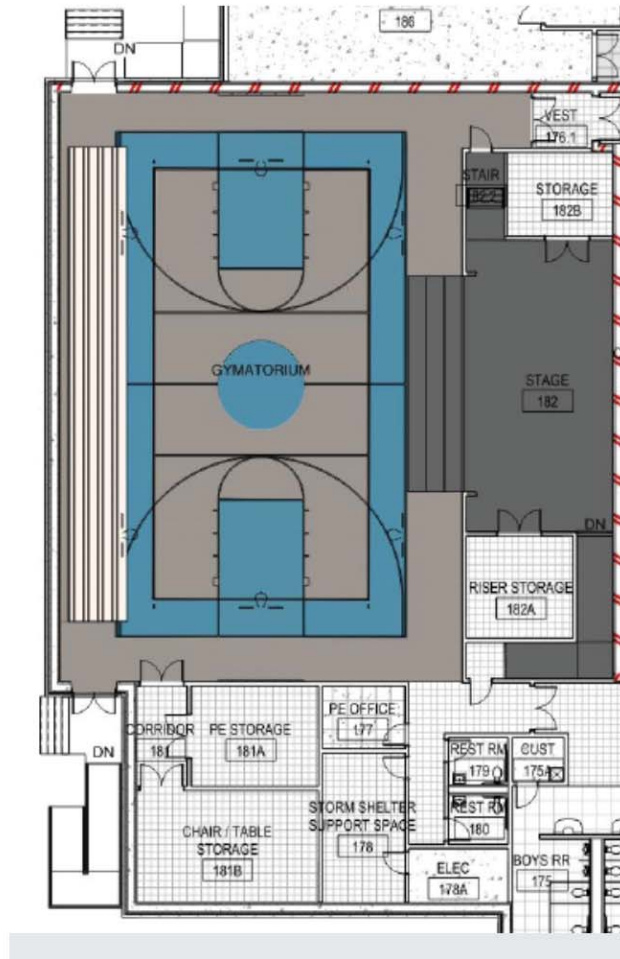
KEY PLAN
