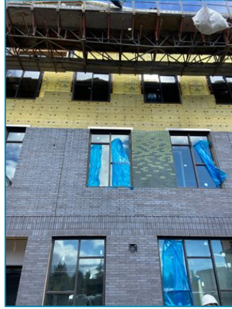
Veneer and glazed brick installation
