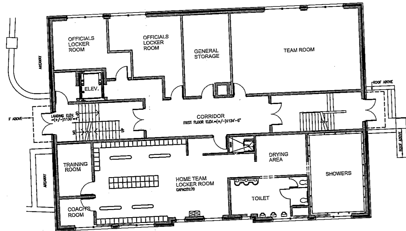
CONCOURSE LEVEL FLOOR PLAN
