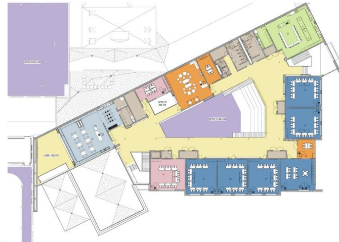
2 OVERALL SECOND FLOOR PLAN 1/8" = 1'-0"
