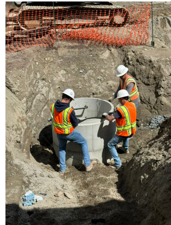
Storm Drain Catch Basin Installation
