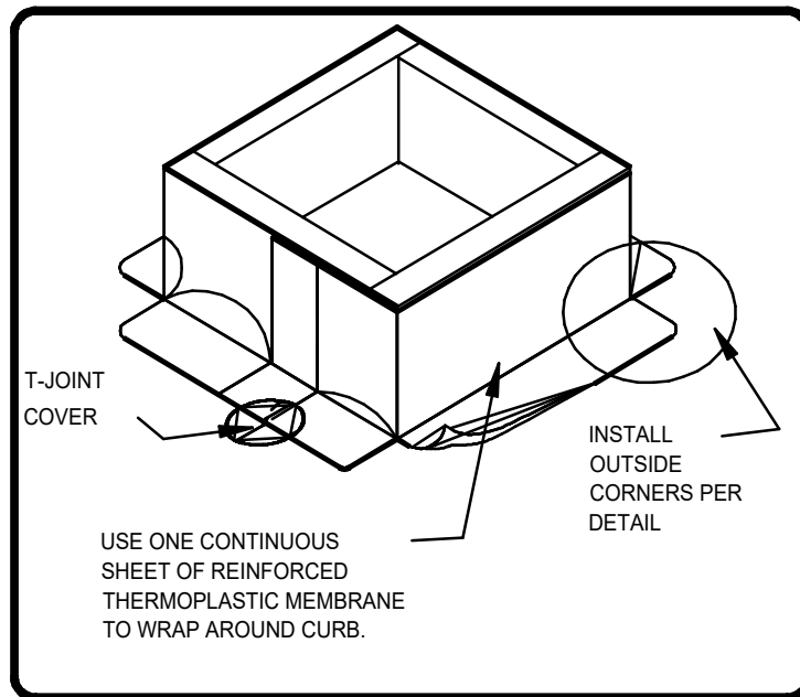
CURB FLASHING
