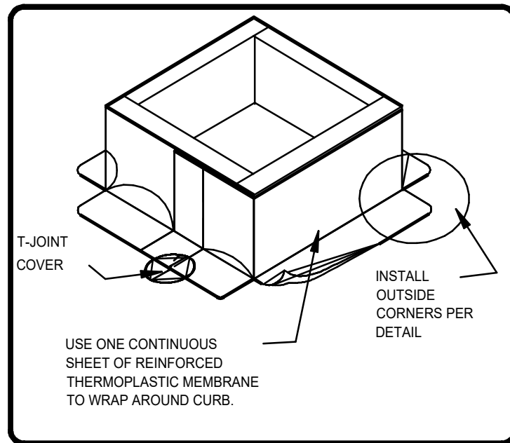
CURB FLASHING
