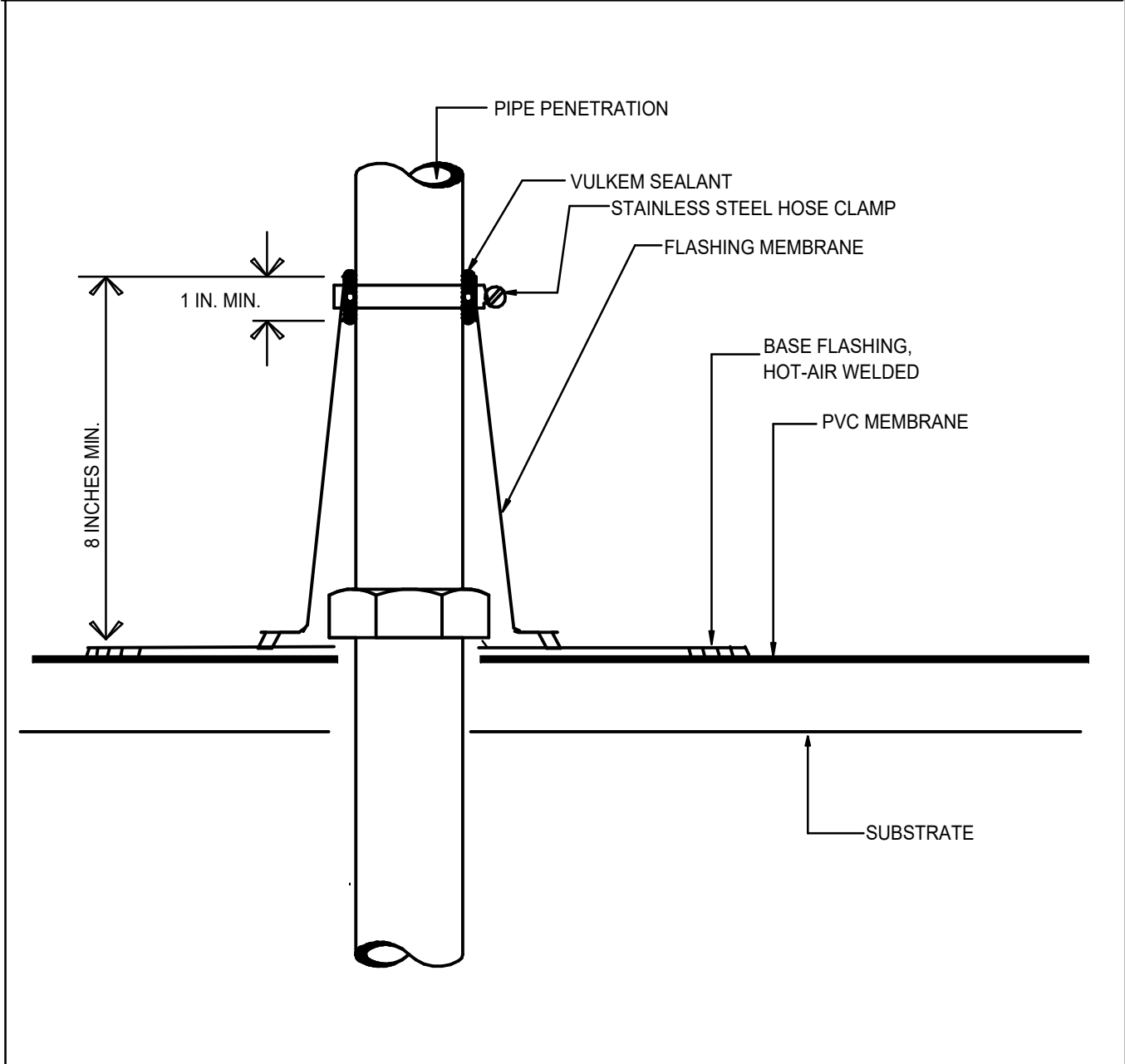
PIPE FLASHING DETAIL
