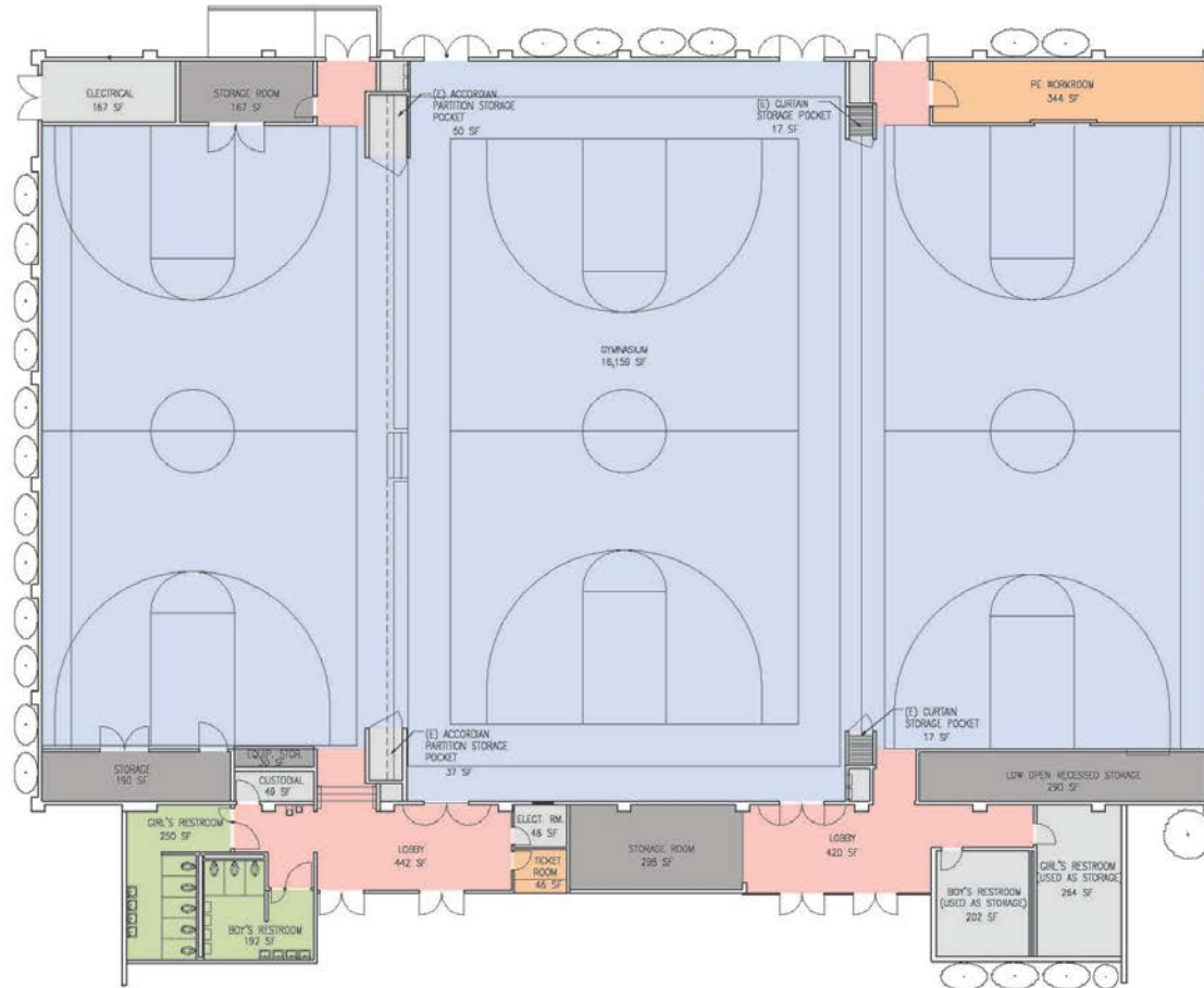
Existing Gymnasium
