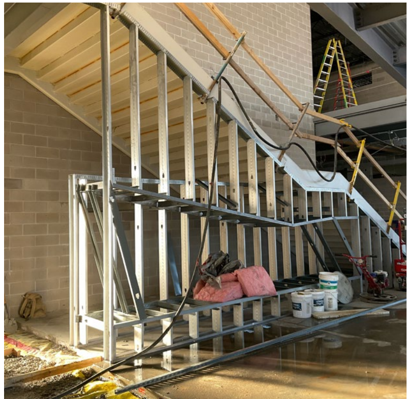
READING NOOK FRAMING INSTALLED UNDER MAIN STAIRWELL
