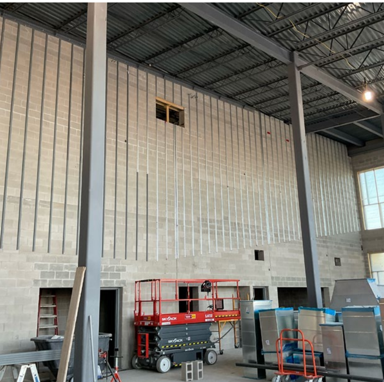
CAFETERIA WALL WITH FURRING STRIPS BEING INSTALLED
