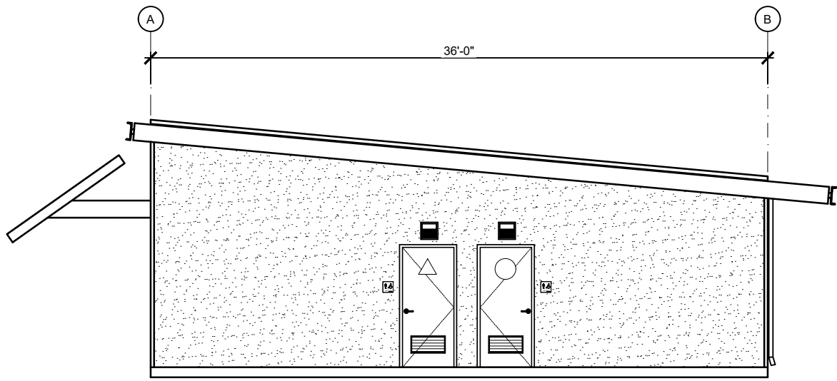
ELEVATION VIEW
