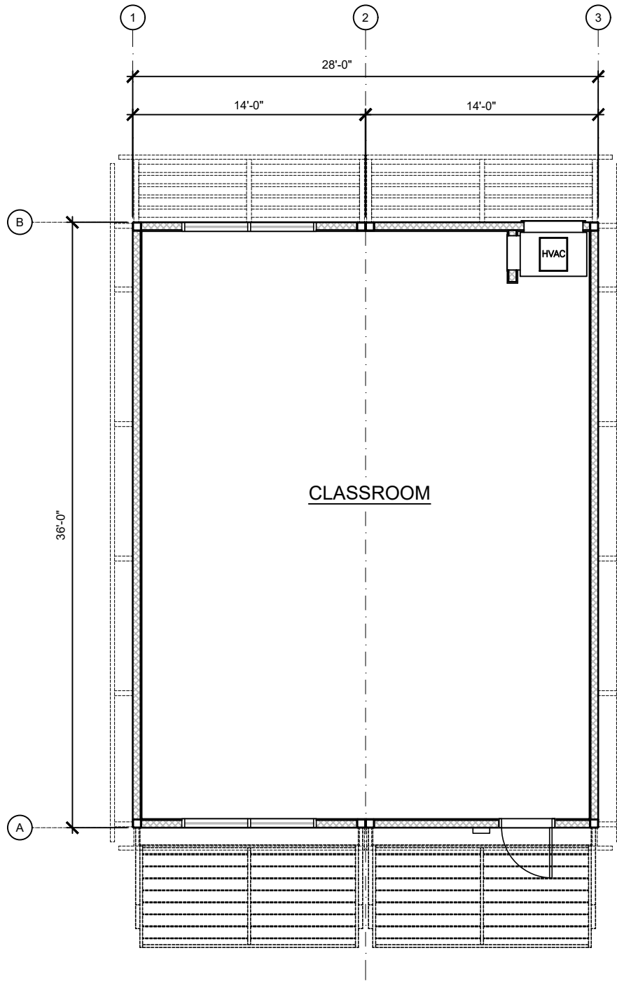
FLOOR PLAN
