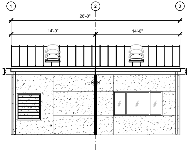
END WALL ELEVATIONS
