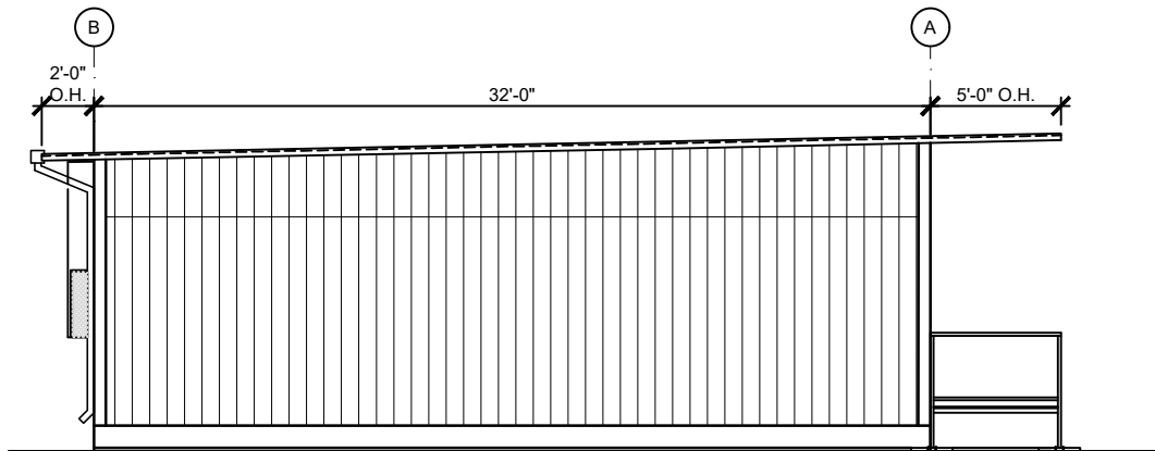
SIDE ELEVATION
