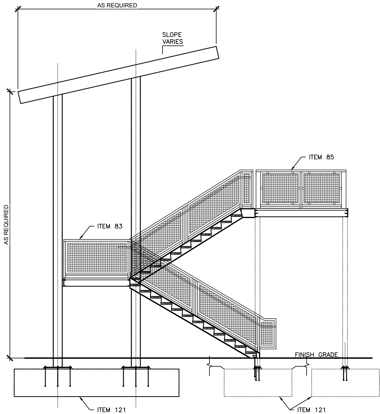
ELEVATION VIEW
