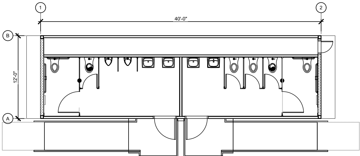
FLOOR PLAN
