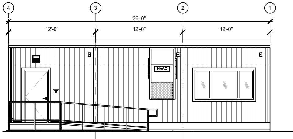
FRONT END/ENTRY ELEVATION
