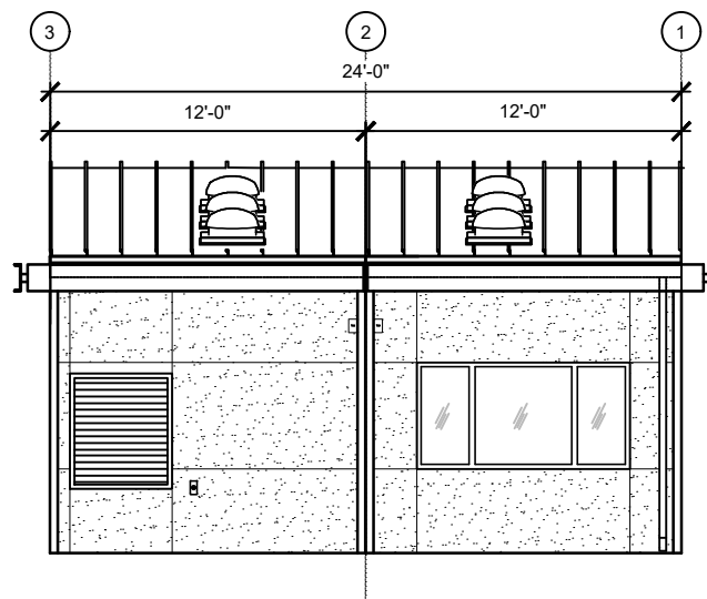
END WALL ELEVATIONS
