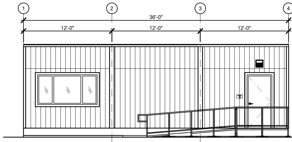
REAR END/ENTRY ELEVATION
