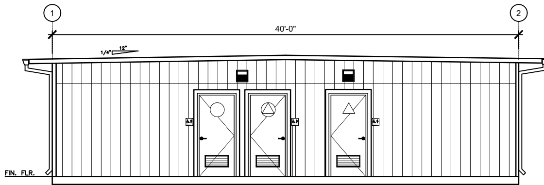
FRONT WALL ELEVATION
