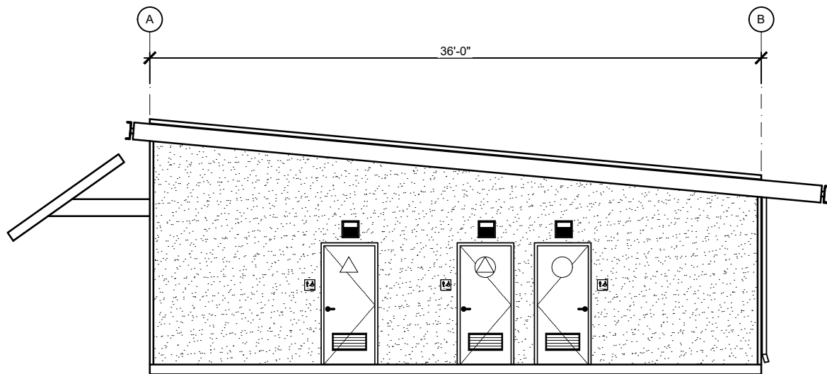
ELEVATION VIEW
