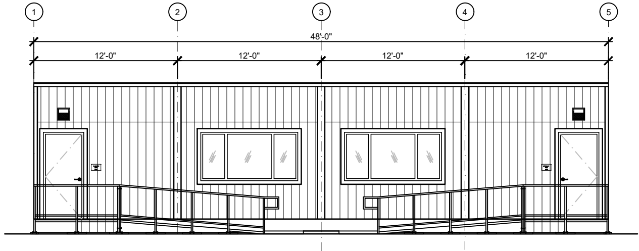
FRONT END/ENTRY ELEVATION
