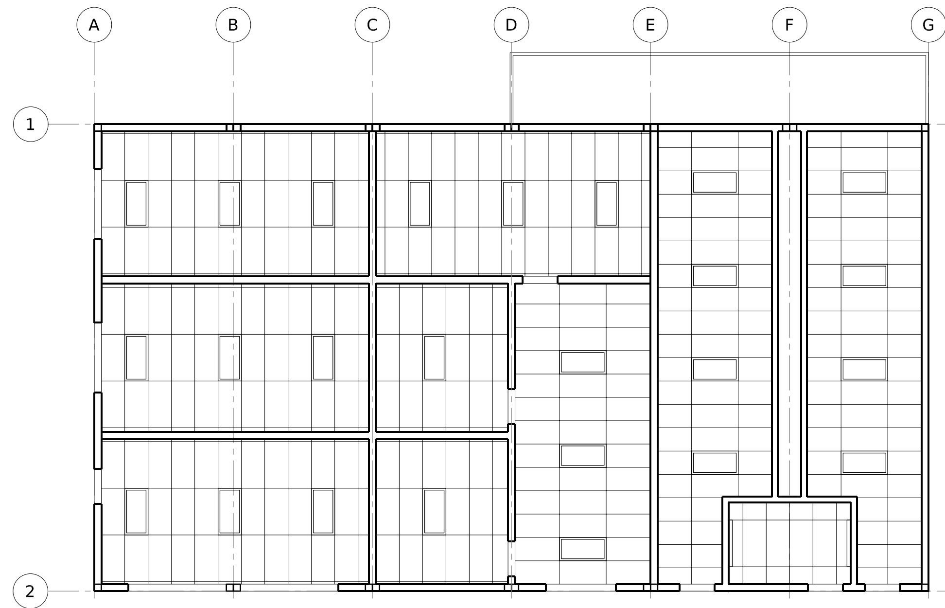
Reflected Ceiling Plan Second Level
