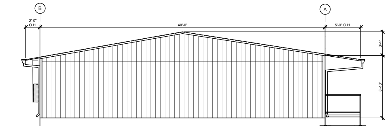
SIDE EXTERIOR ELEVATION
