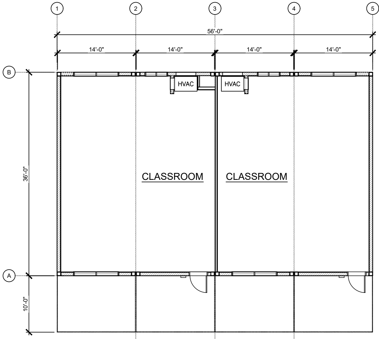
SECOND FLOOR PLAN VIEW
