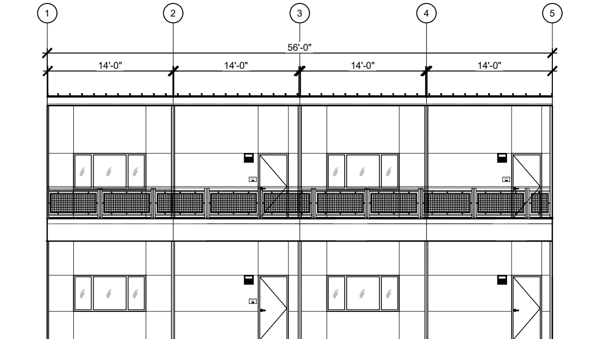
FRONT ELEVATION
