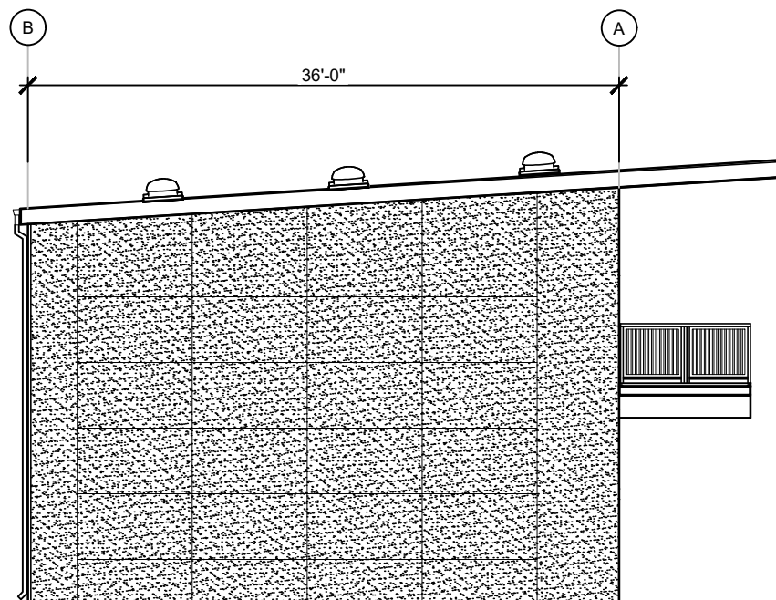
FRONT ELEVATION
