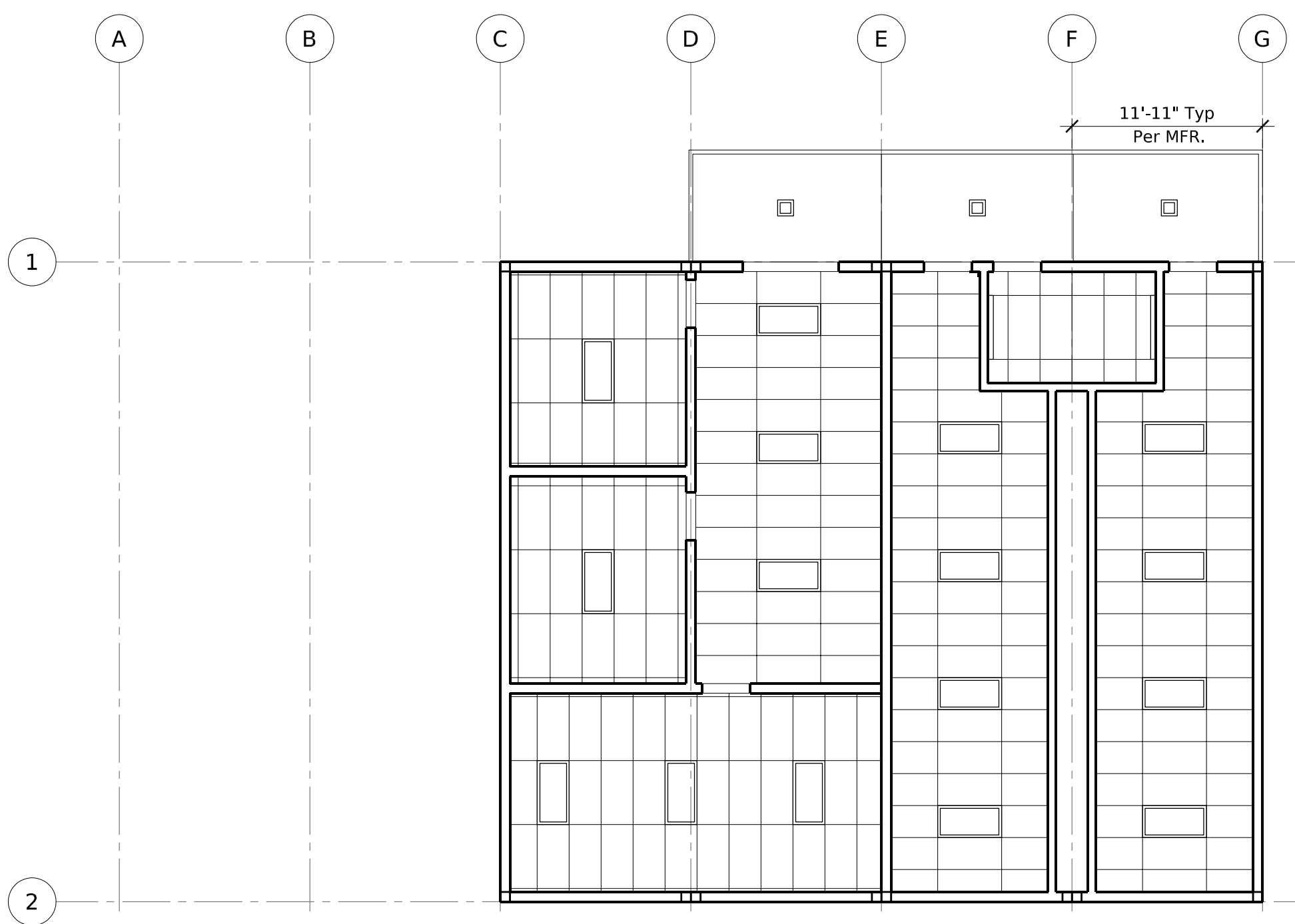
Reflected Ceiling Plan Second Level
