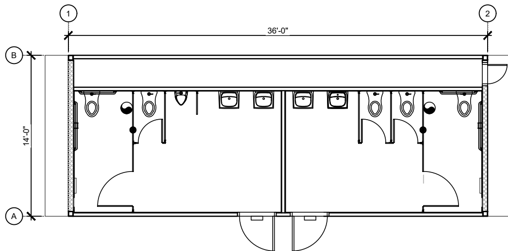
FLOOR PLAN
