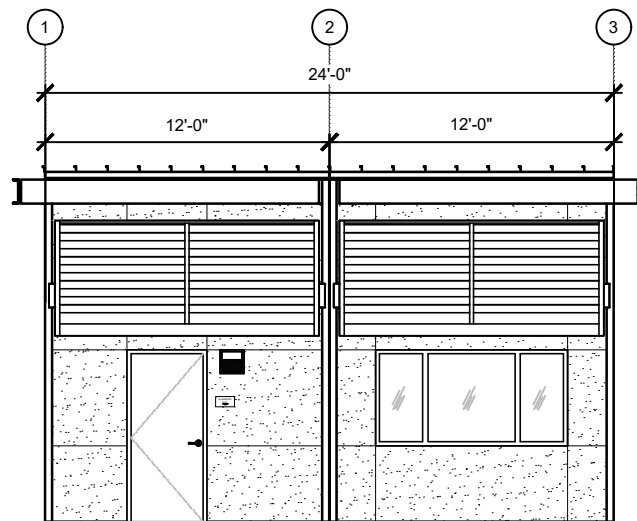
FRONT WALL ELEVATION
