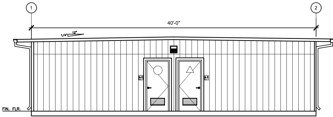
FRONT WALL ELEVATION
