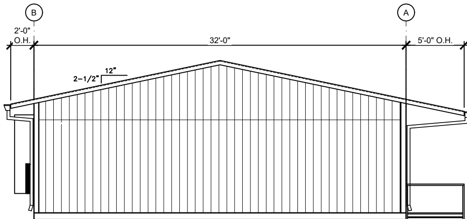
SIDE EXTERIOR ELEVATION
