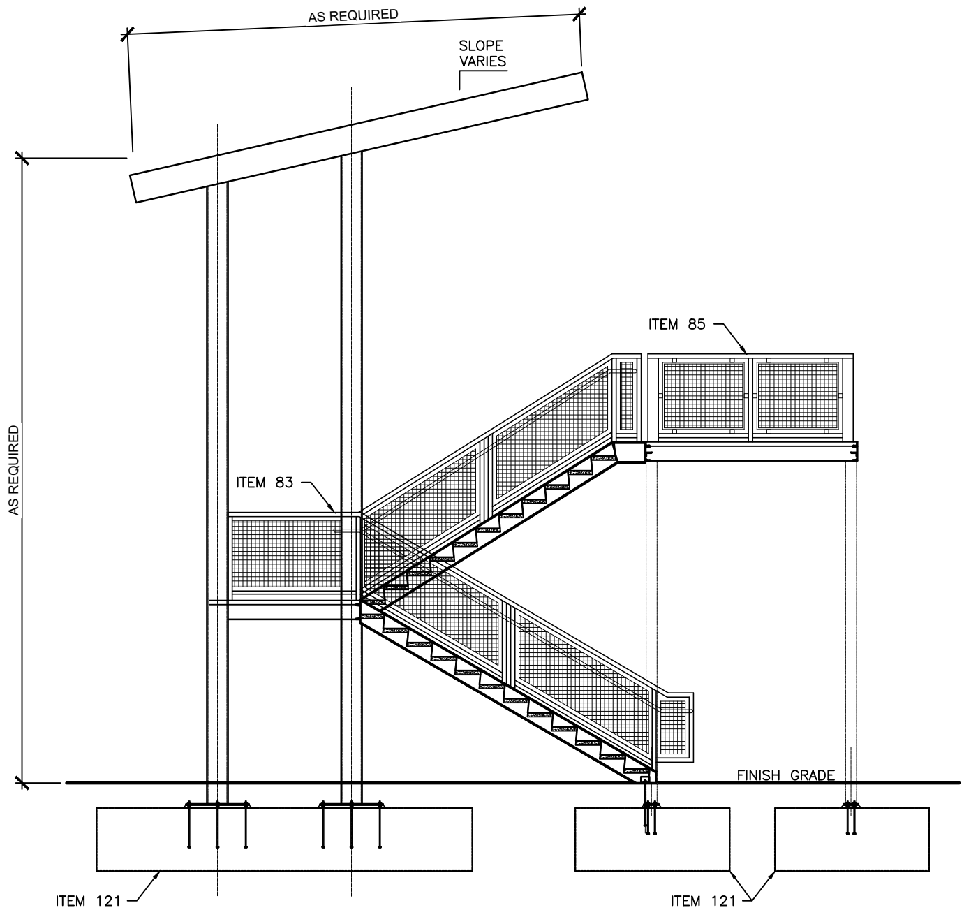
ELEVATION VIEW
