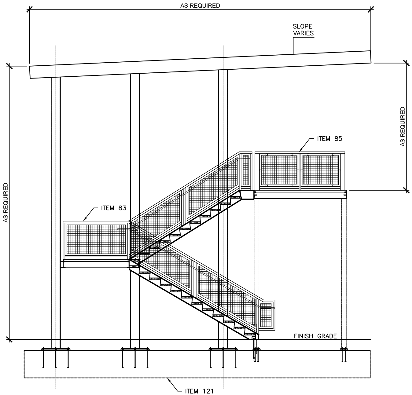
ELEVATION VIEW
