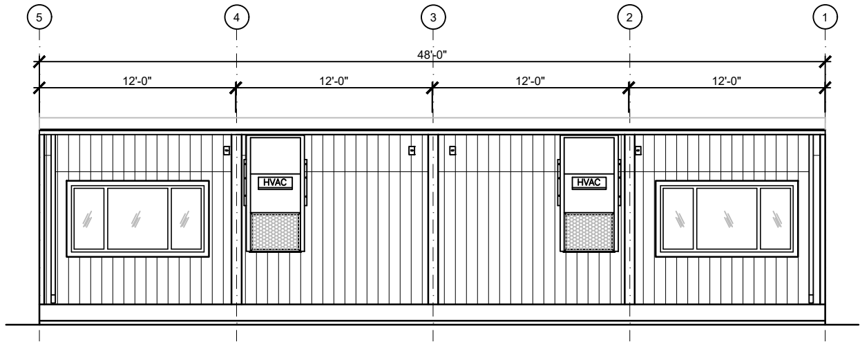
REAR END/ENTRY ELEVATION
