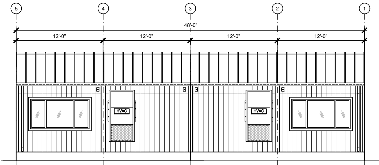
REAR EXTERIOR ELEVATION
