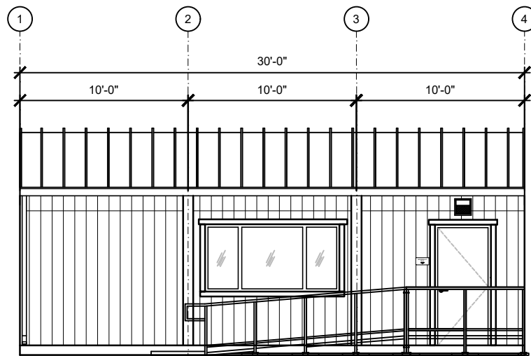
FRONT EXTERIOR ELEVATION
