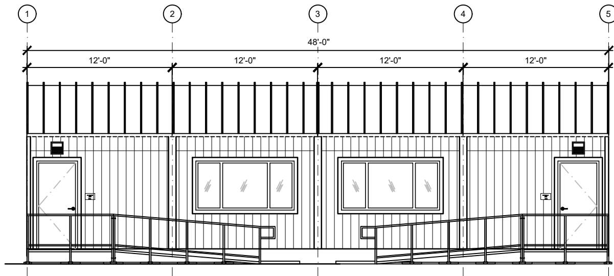
FRONT EXTERIOR ELEVATION
