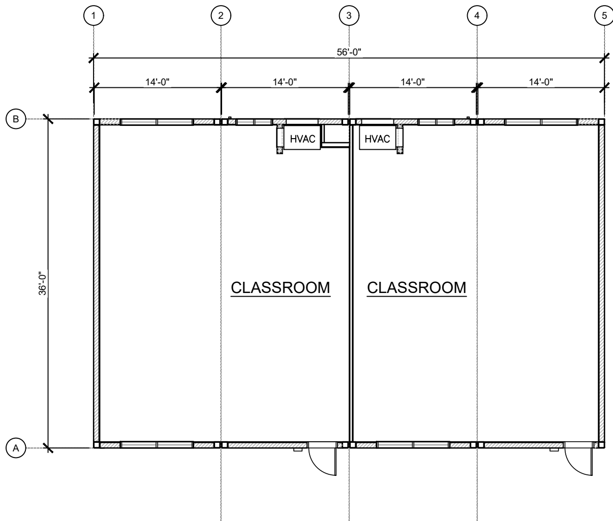
FIRST FLOOR PLAN VIEW
