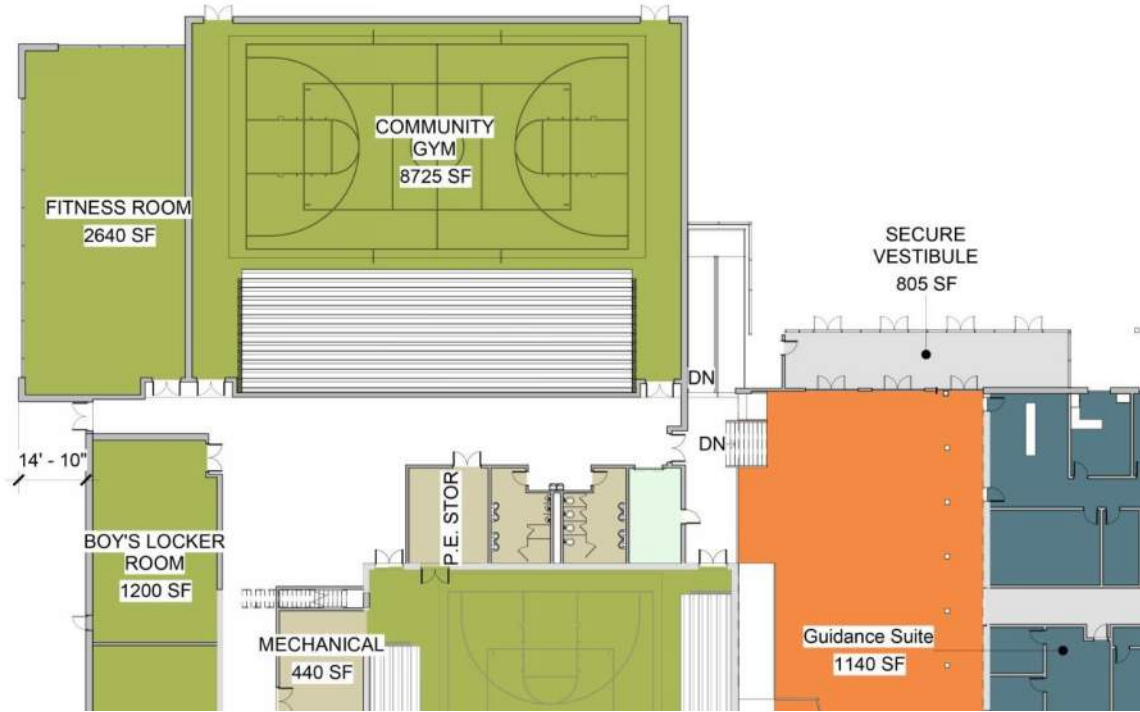
ALTERNATE 1 – GYM TO REPLACE SLC
