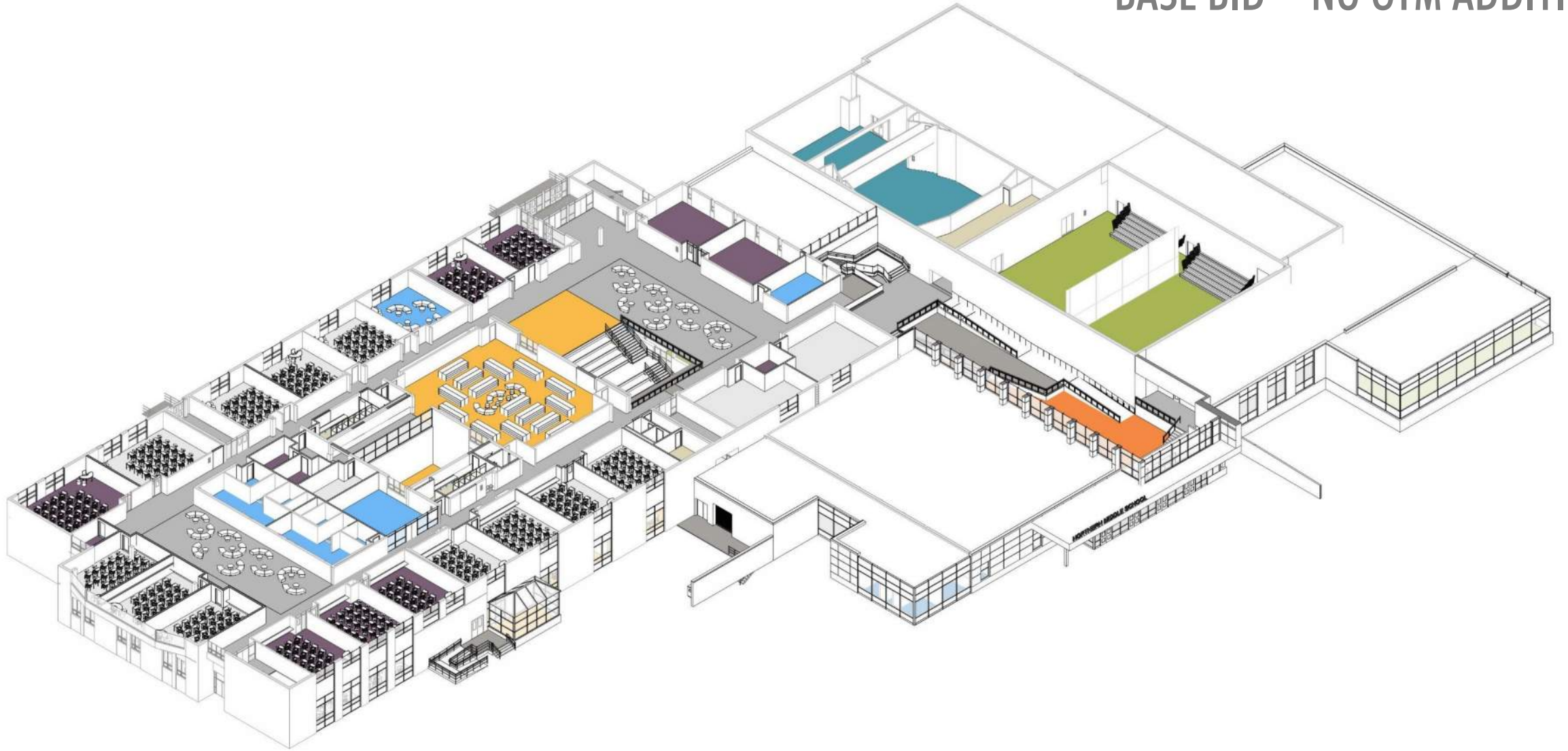
PROPOSED SECOND FLOOR
