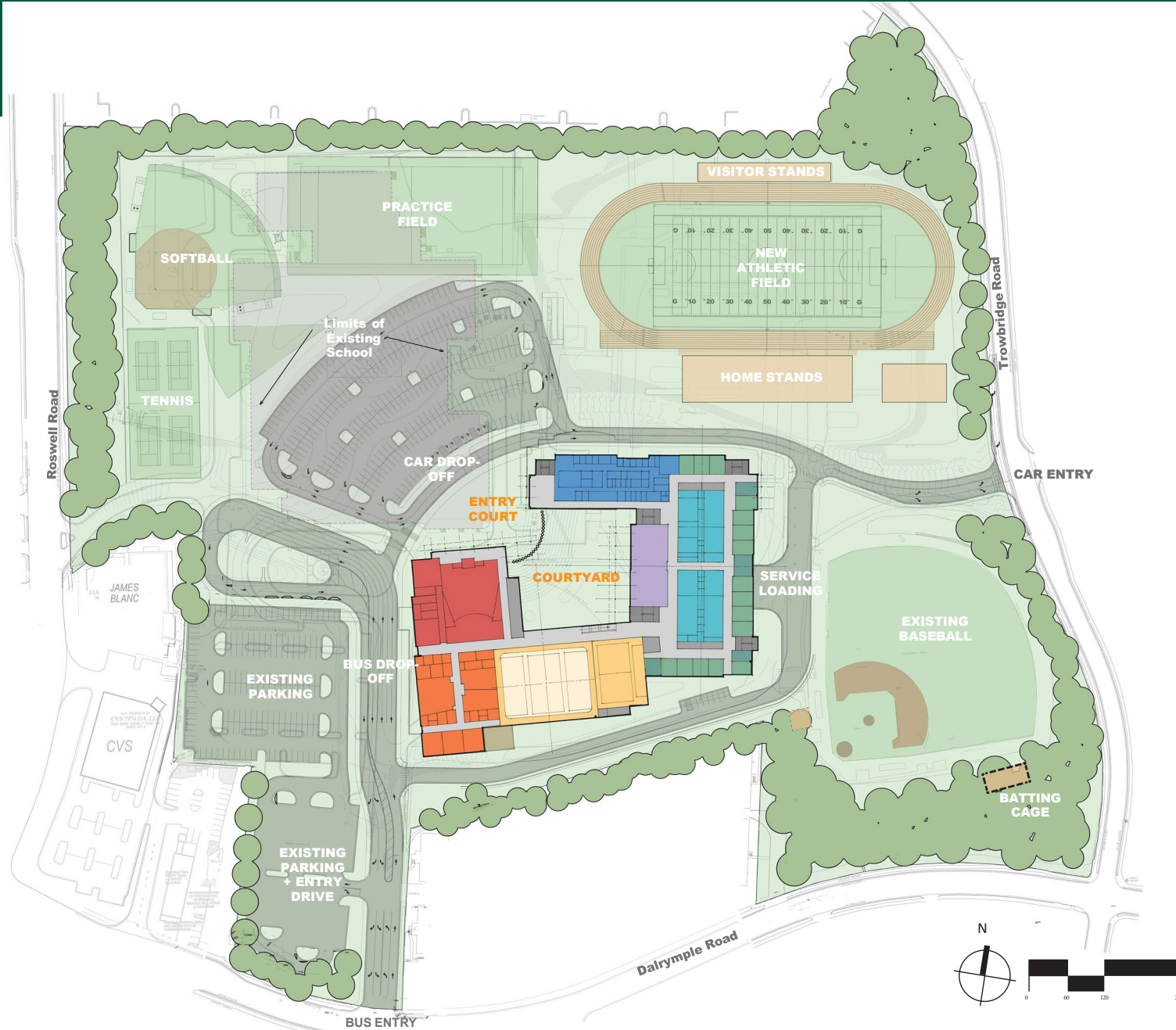
SITE PLAN
