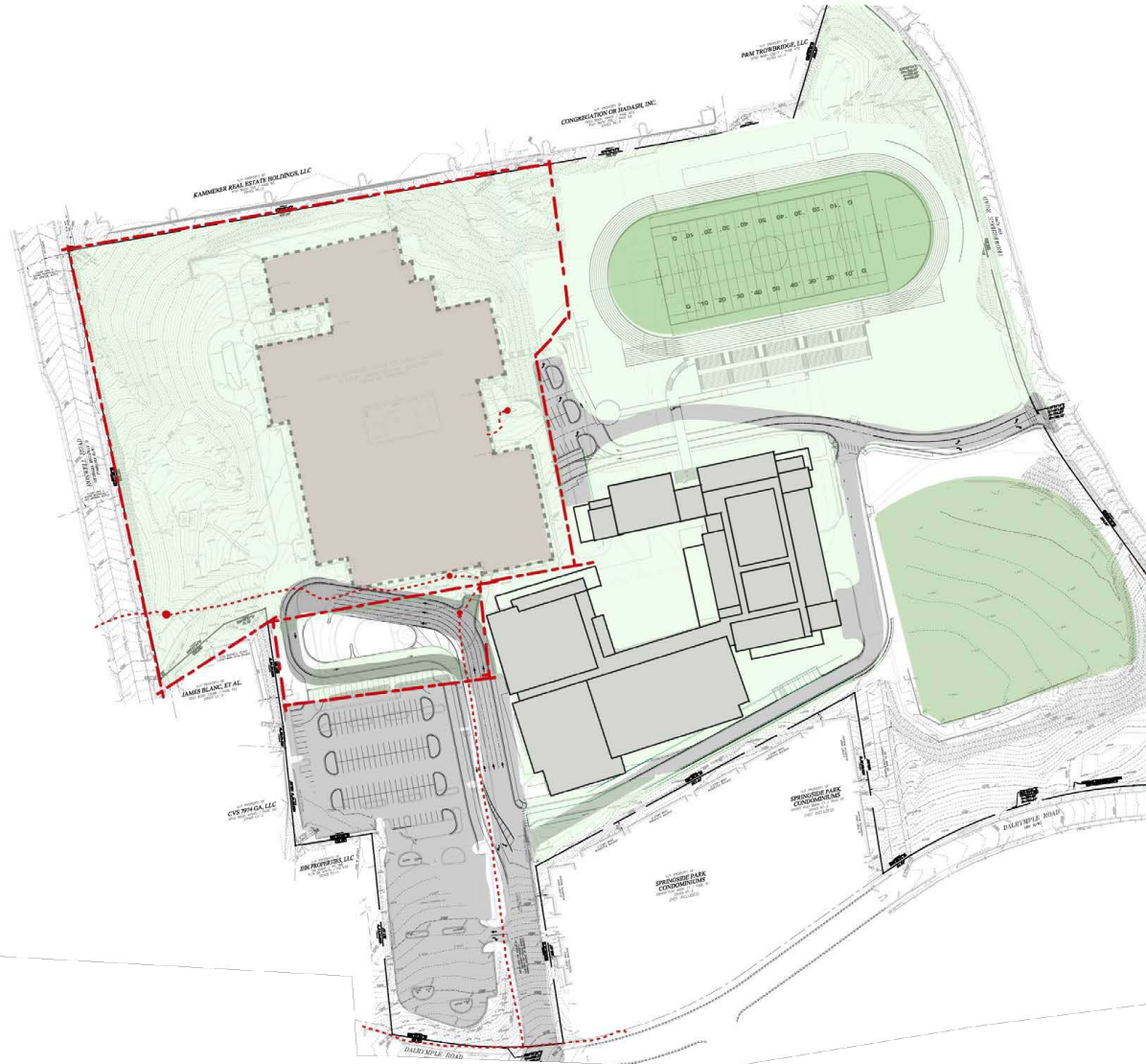
PHASE 2 - BUS AND DRIVES
