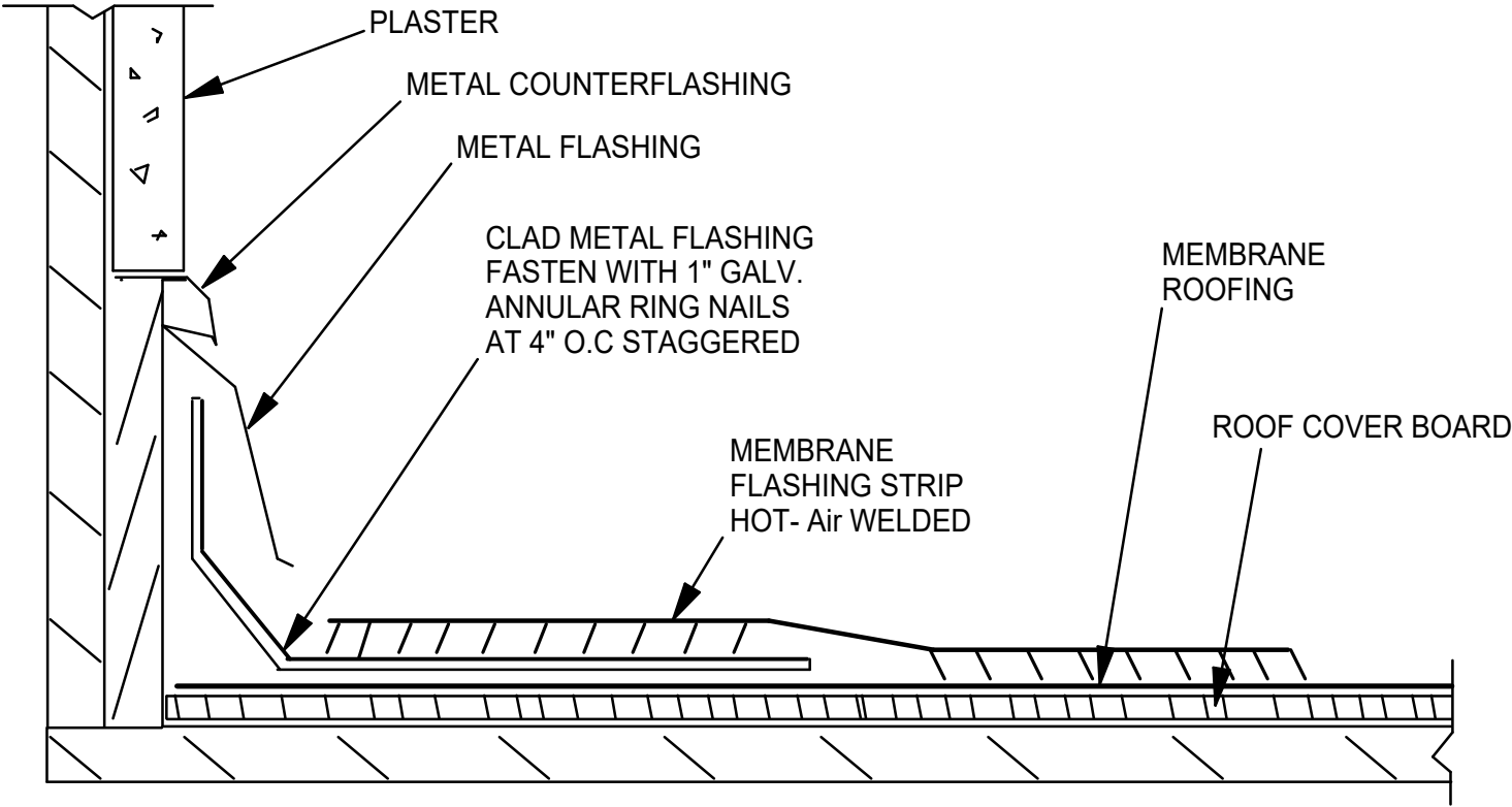
LOW FLASHING DETAIL
