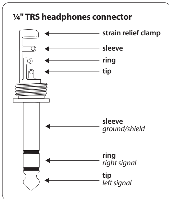
Stereo plug for headphones connection
