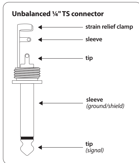
1/4" mono plug
