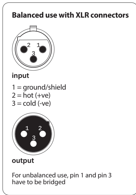
XLR connections
