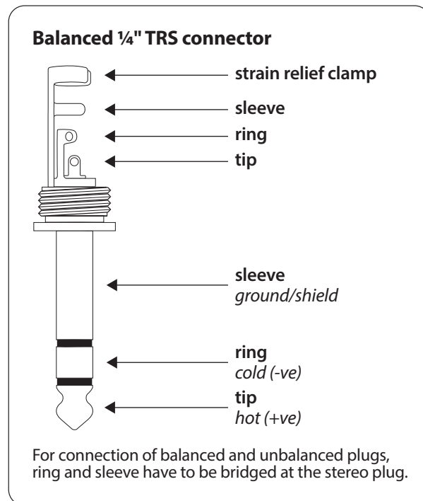
1/4" stereo plug
