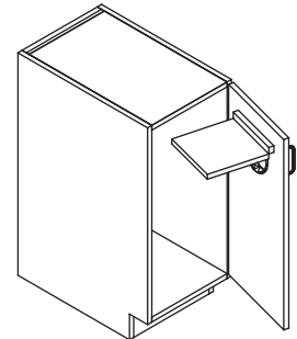
WASTE CABINET WITH 6" ROUND DOOR GROMMET WITH REAR FLAP, HINGED RIGHT
