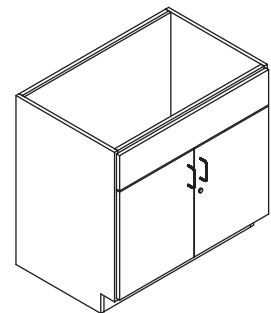
SINK CABINET 2 HINGED DOORS WITH LOCK, OPEN TOP
