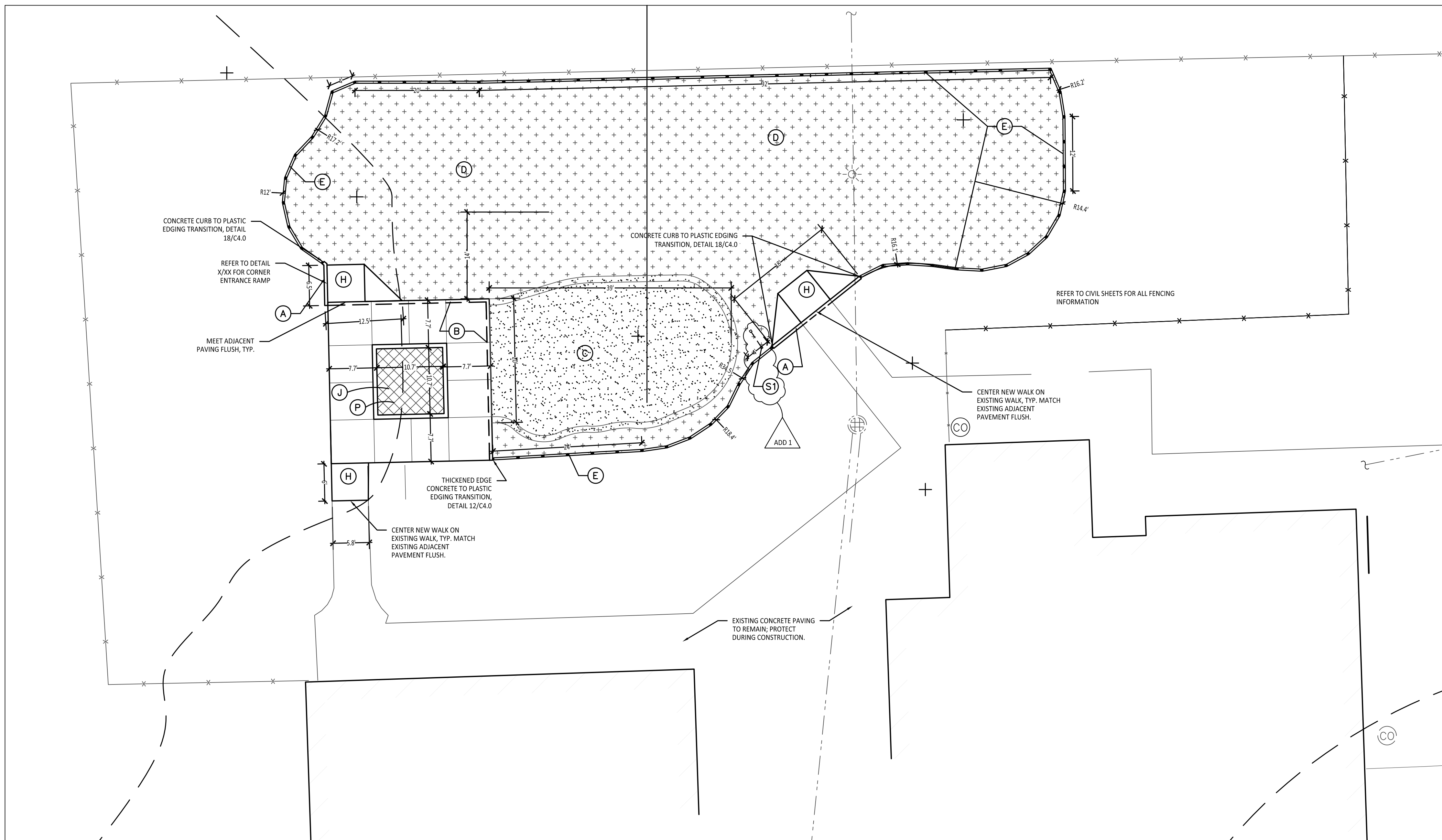
1 Playground Layout Enlargement Plan -- Kindergarten + 1st Grade 1" = 10'-0"
