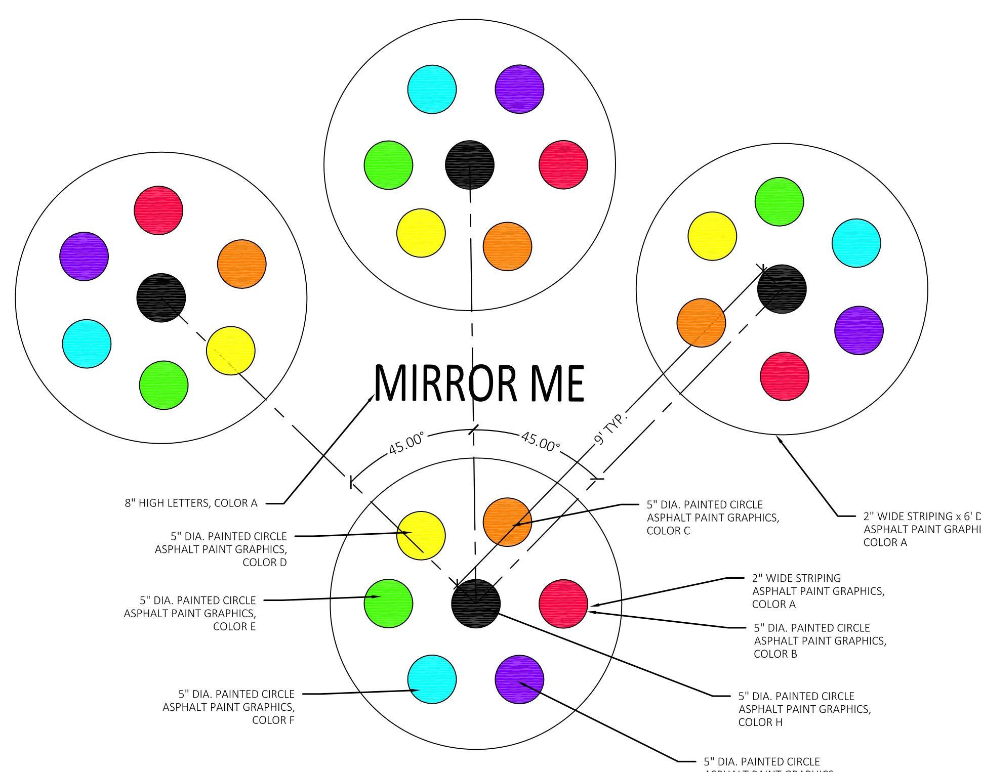
2 Mirror Me Detail Not to Scale
