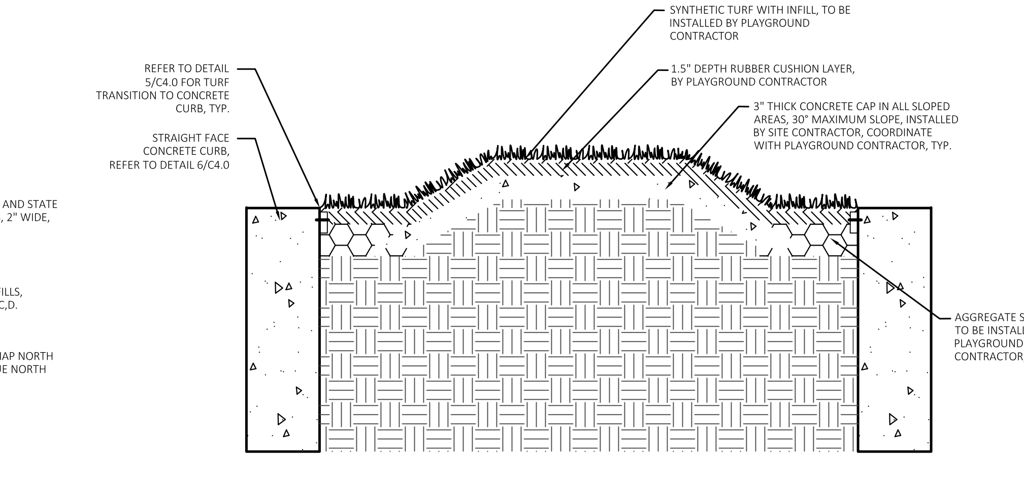
4 Synthetic Turf Mound Detail Not to Scale
