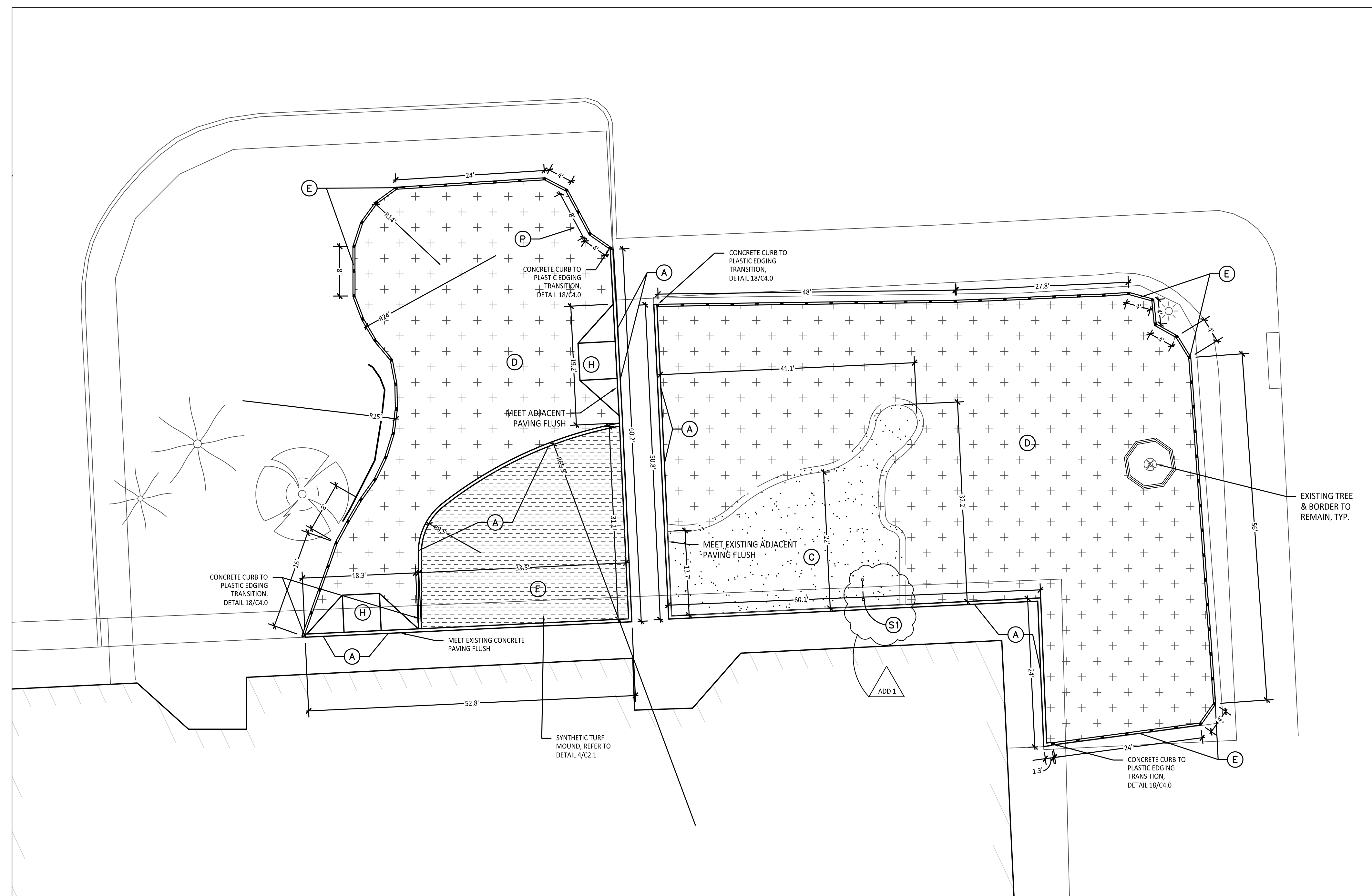
1 Playground Layout Enlargement Plan - Kindergarten Scale: 1" = 10'-0"
