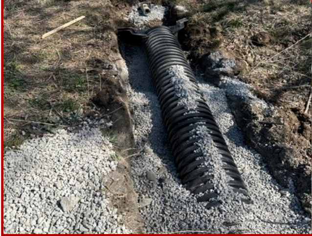
Extend Drainage Pipe to Retention Area
