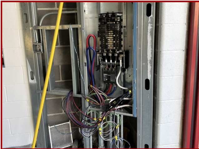
Panelboard in Auxiliary Classroom
