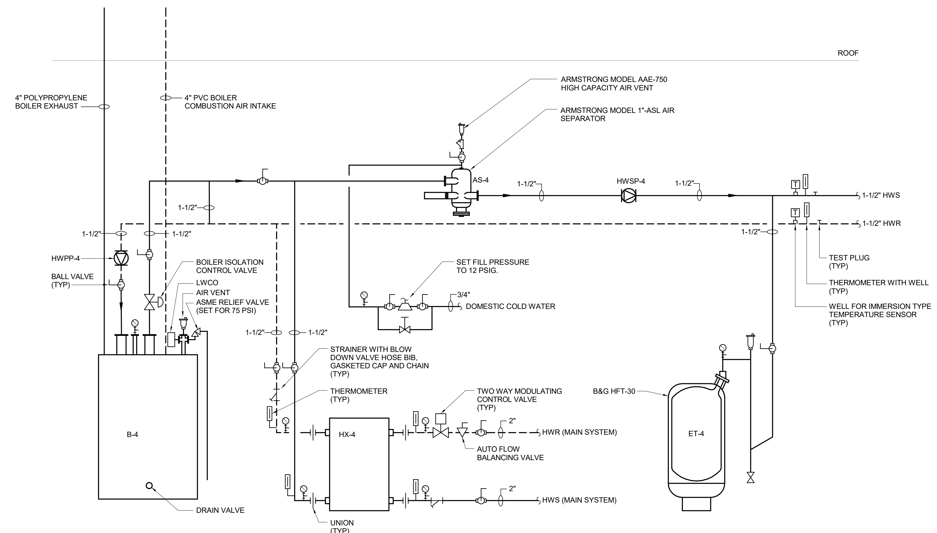
2 PROPOSED HOT WATER HEATING SYSTEM PIPING SCHEMATIC - B-4 NOT TO SCALE
