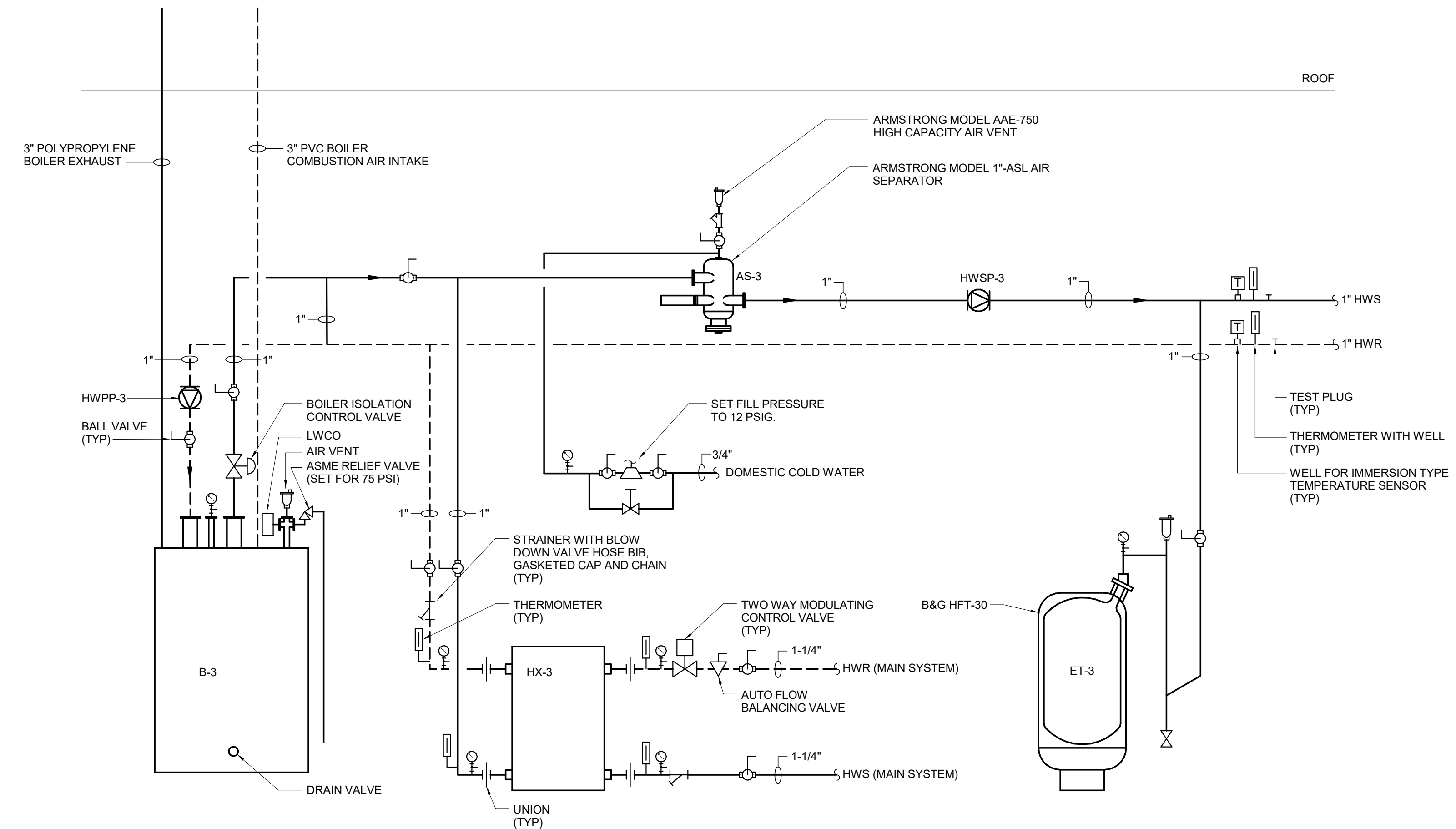
1 PROPOSED HOT WATER HEATING SYSTEM PIPING SCHEMATIC - B-3 NOT TO SCALE
