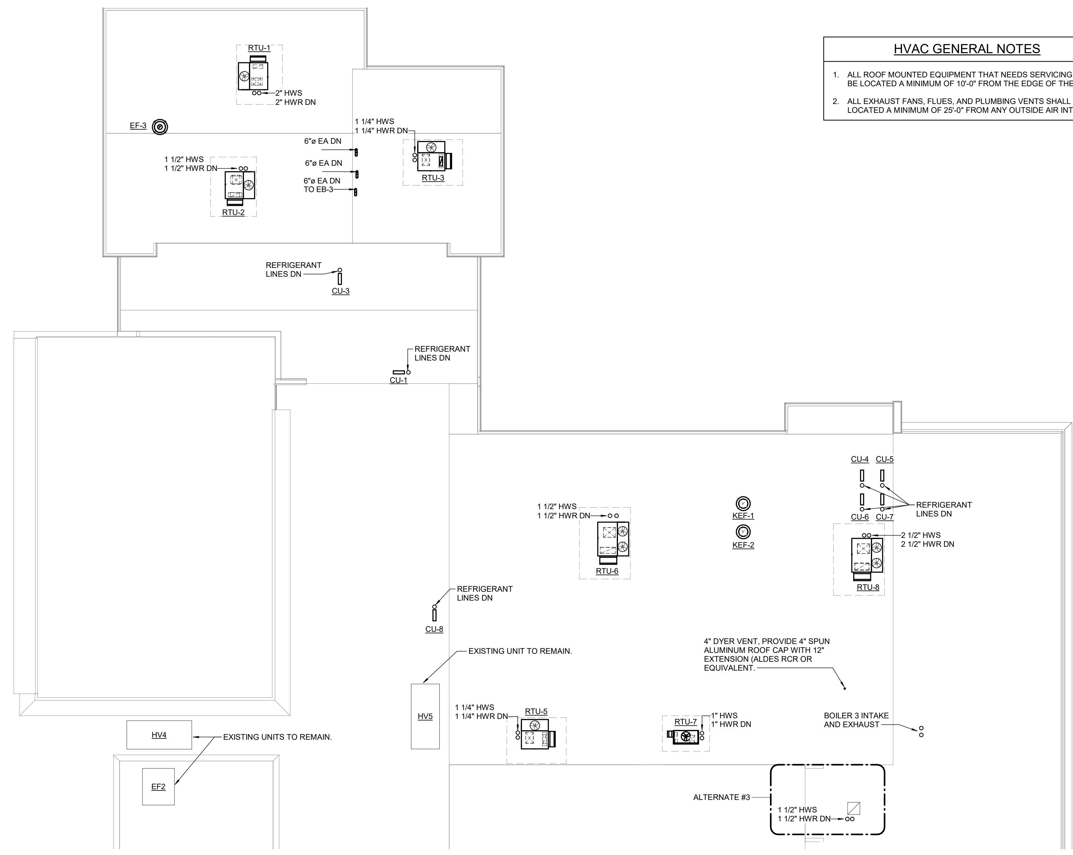
1 ROOF PLAN AREA A,B,&E 1/16" = 1'-0"
