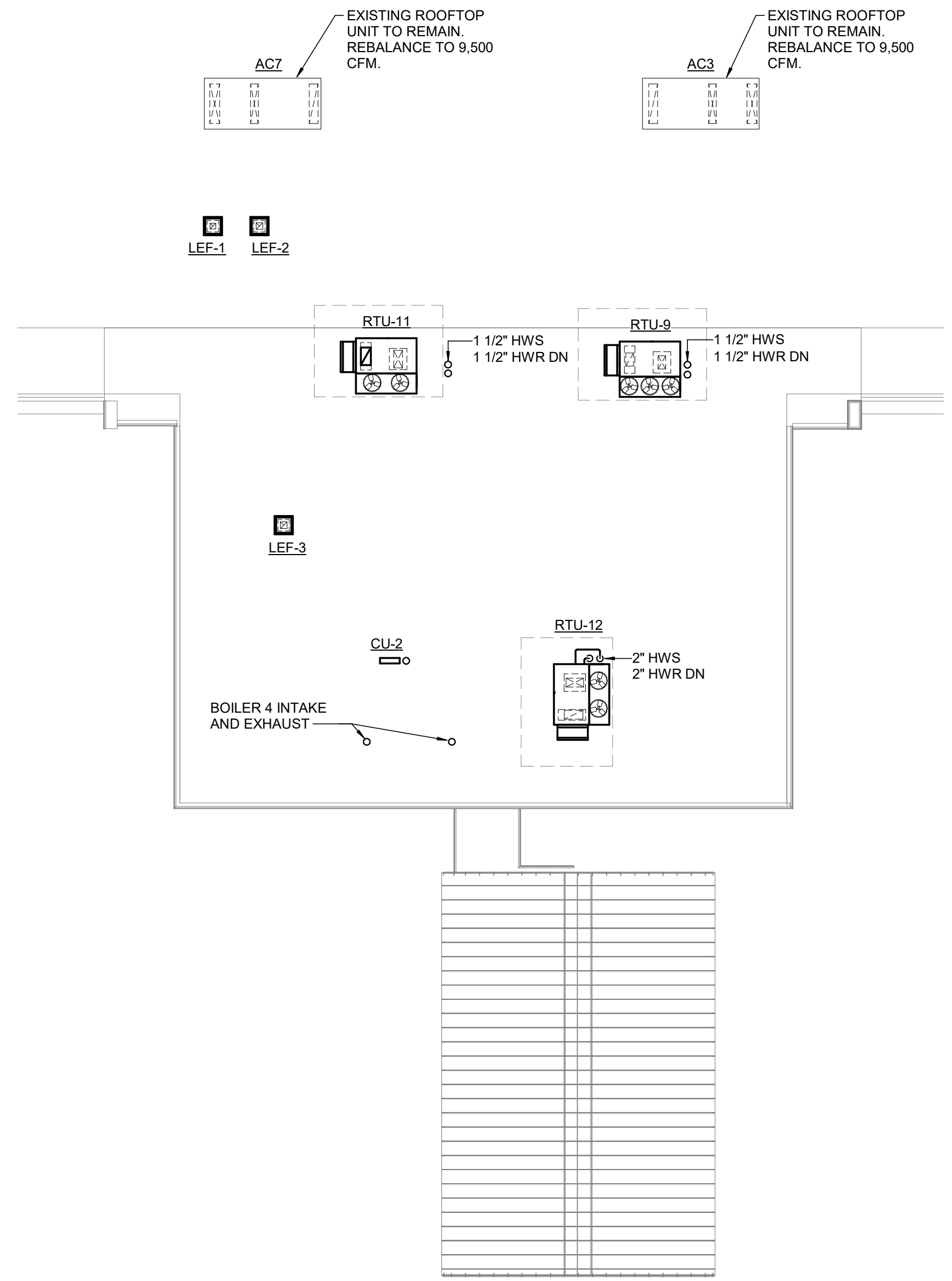
2 ROOF PLAN AREA C,D,&E 1/16" = 1'-0"
