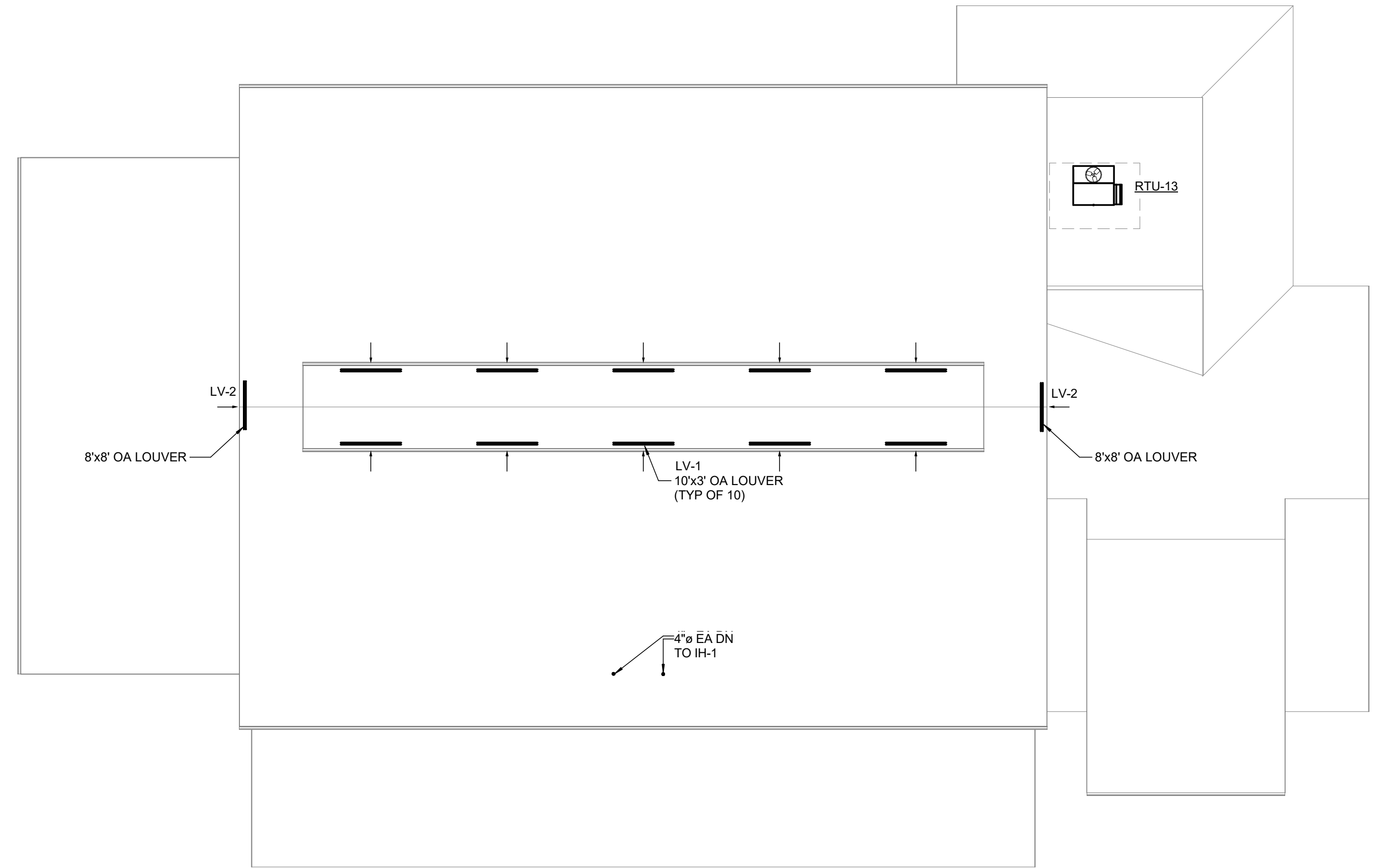
3 ROOF PLAN - AREA F 1/16" = 1'-0"
