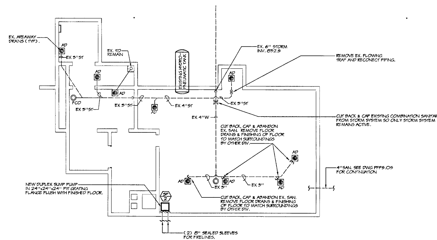
1 PLUMBING/FIRE PROTECTION LOWER LEVEL UNDERGROUND FLOOR PLAN- AREA D SCALE: 1/8"=1'-0" NOTES: 1. SEE SYMBOLS, SCHEDULES, NOTES AND DETAILS.
