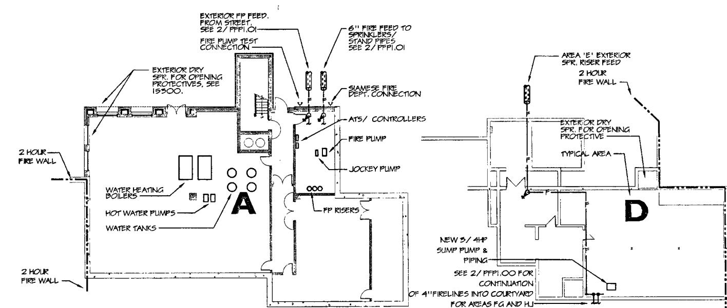
1 PLUMBING/FIRE PROTECTION LOWER LEVEL PART FLOOR PLANS SCALE: 1/16" = 1'-0"
