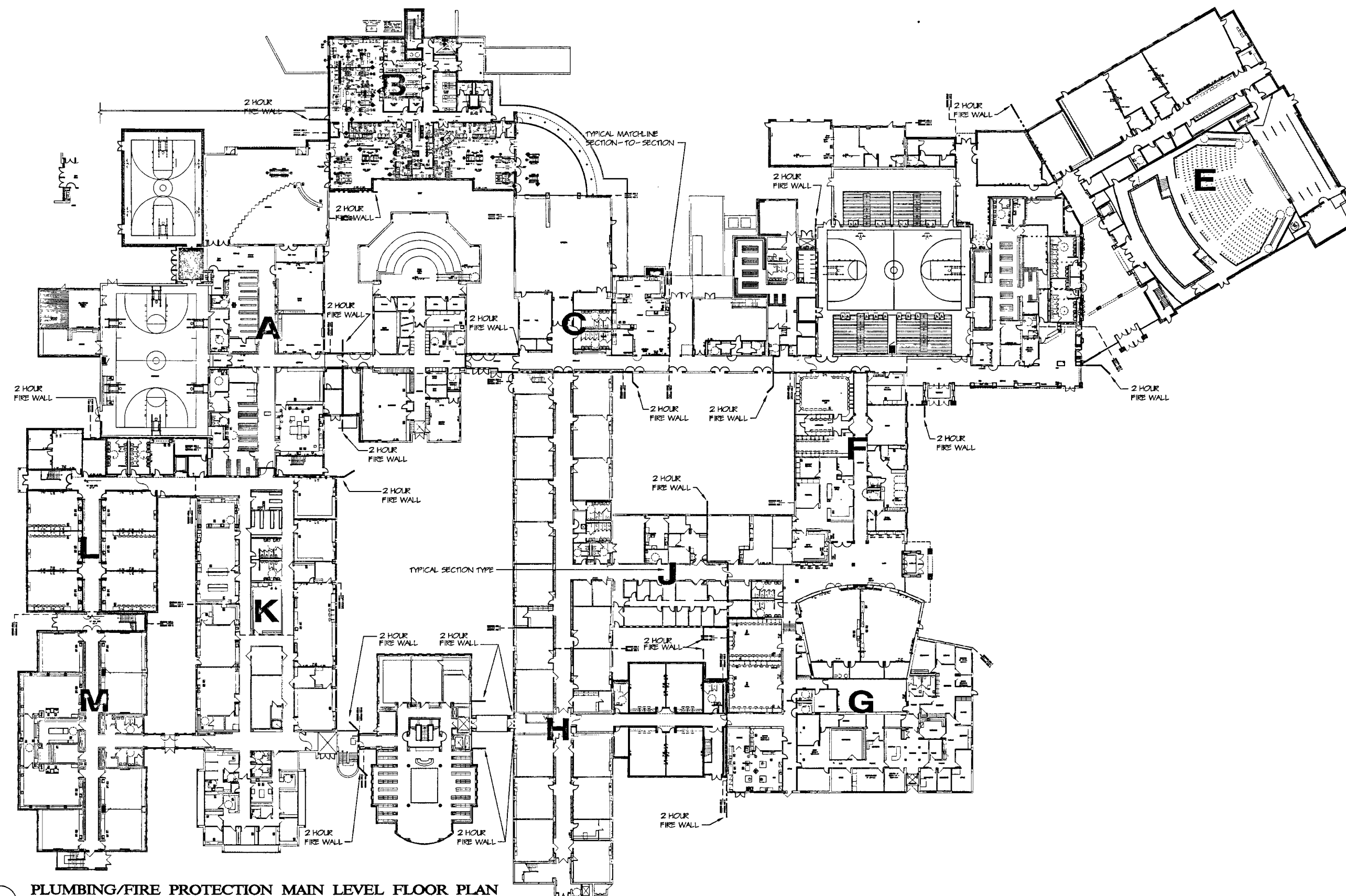
2 PLUMBING/FIRE PROTECTION MAIN LEVEL FLOOR PLAN
