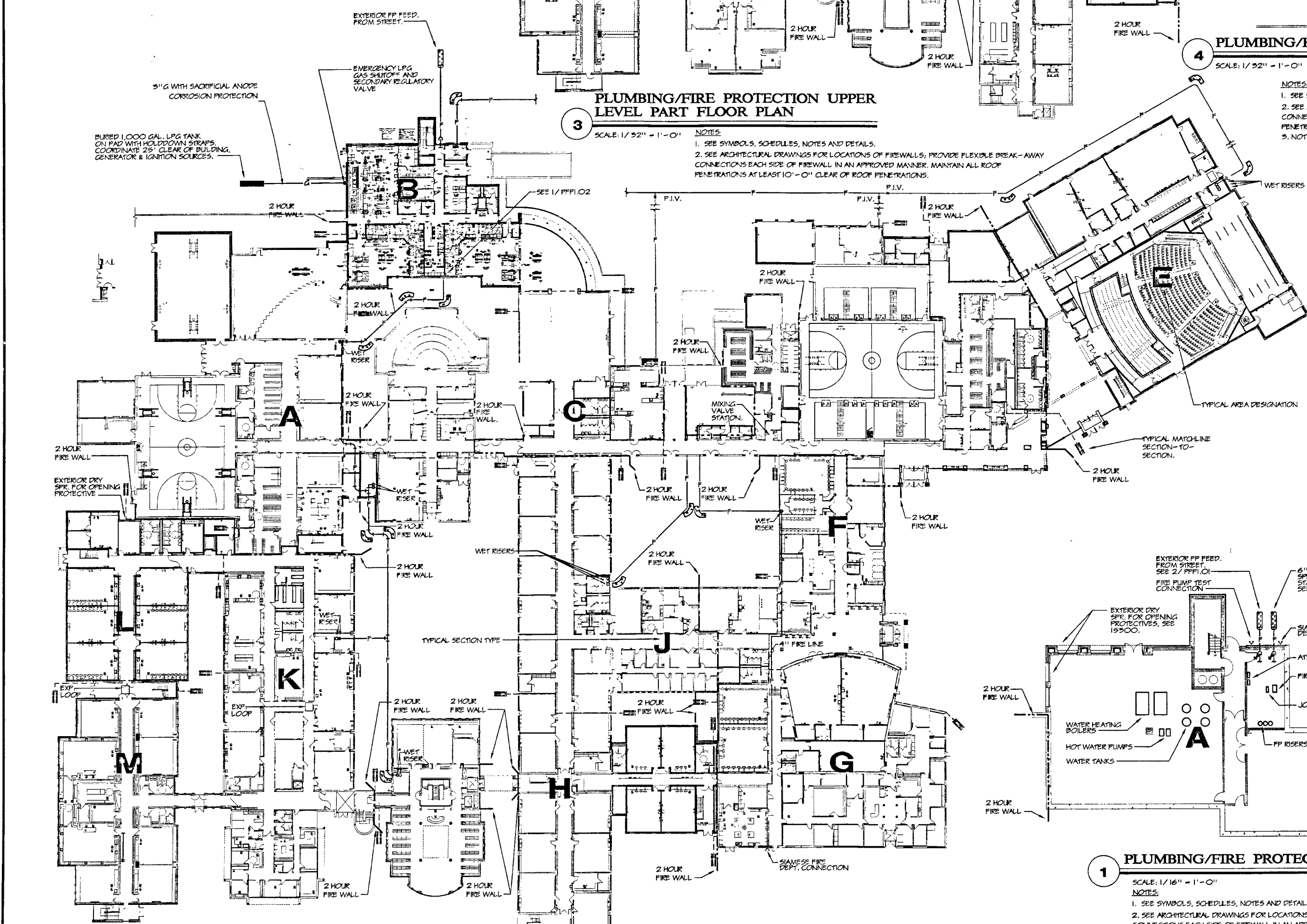
2 PLUMBING/FIRE PROTECTION MAIN LEVEL FLOOR PLAN SCALE: 1/32" = 1'-0"
