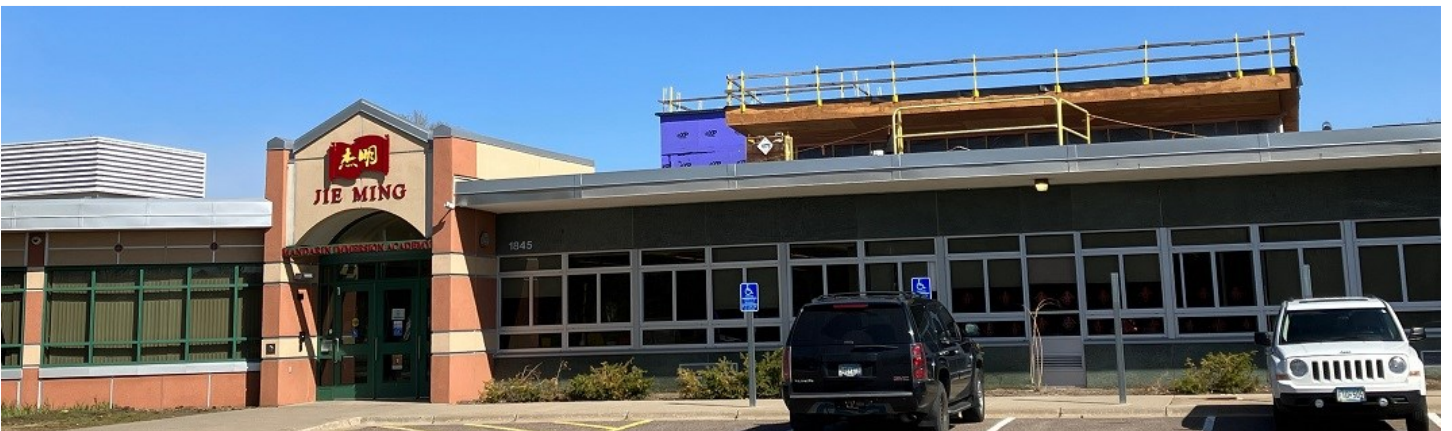
From top to bottom, left to right: Mechanical, electric and plumbing rough-ins in kitchen; interior wall framing in classrooms; concrete floor slabs are complete; mechanical penthouse stair; cafeteria addition from front of school (April 2023)
