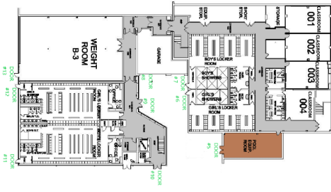
Basement Level Floor Plan Scale: 1" = 50'-0"
