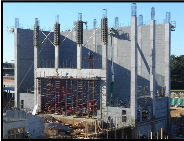
Auditorium Structure
