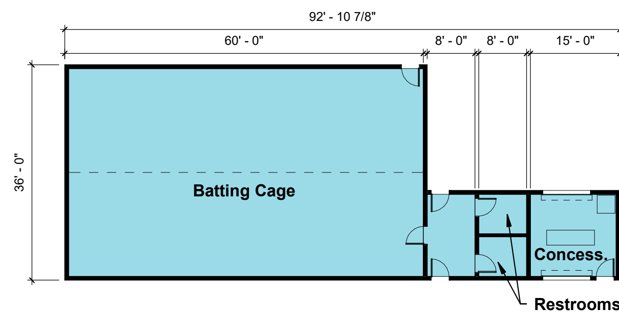
NORTH Concession/Batting Cage Floor Plan 1/16" = 1'-0" 0 8 16 32
