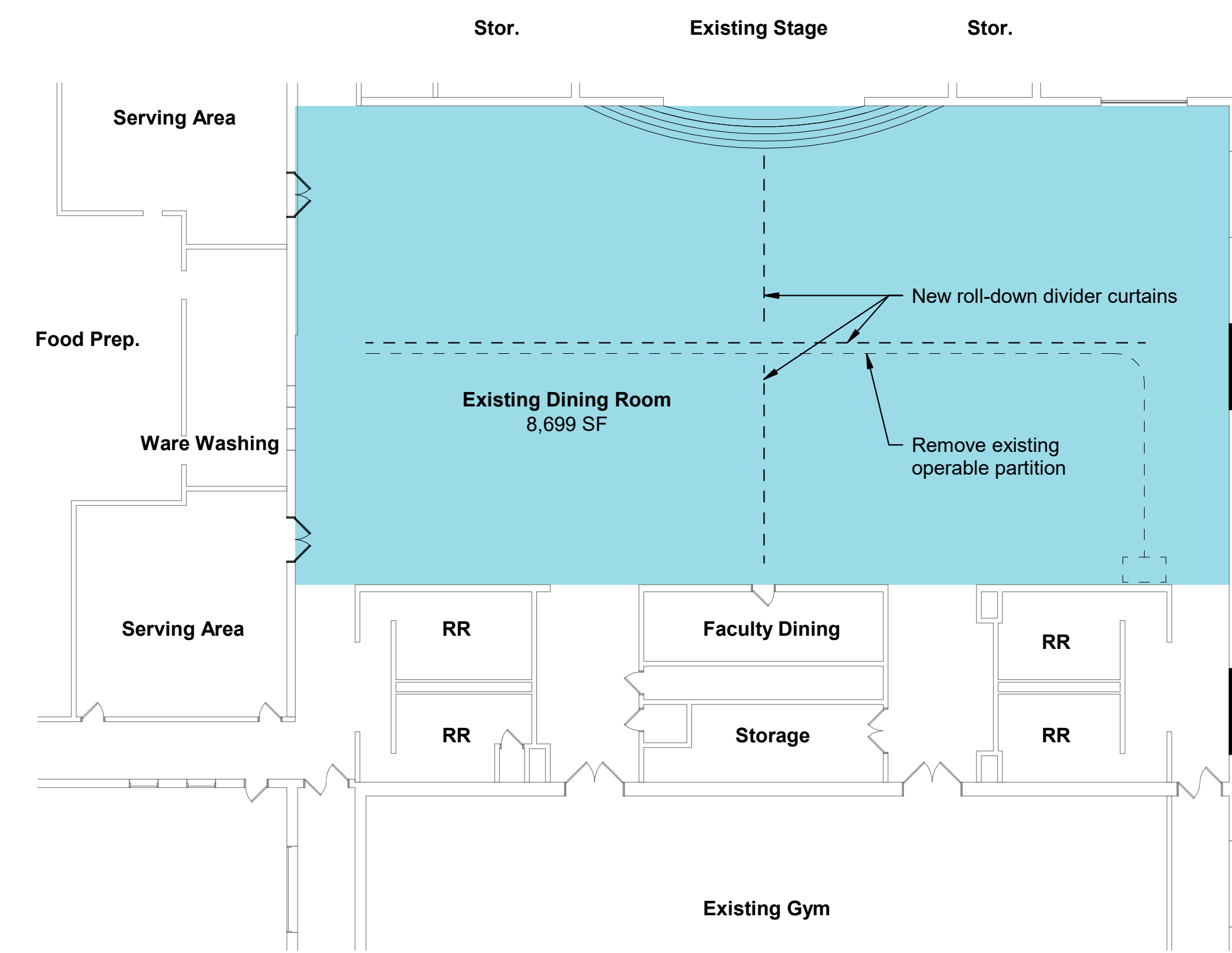
NORTH 3-12 Dining Room Renovation First Floor Plan 1/16" = 1'-0"
