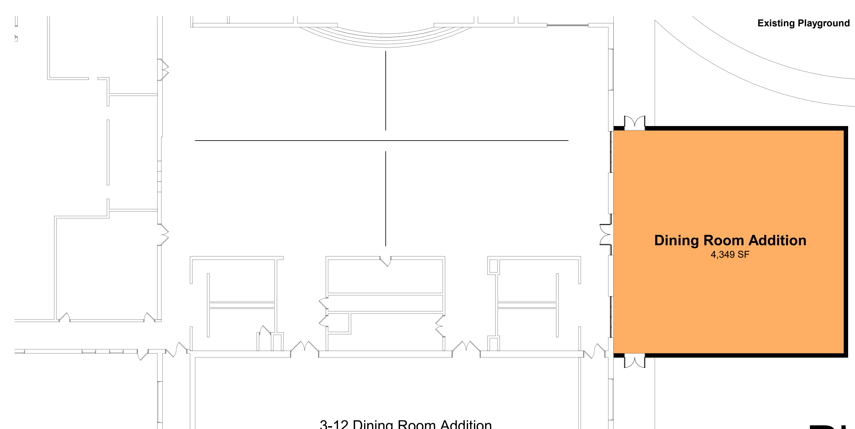
NORTH 3-12 Dining Room Addition First Floor Plan 1/16" = 1'-0" 0 8 16 32
