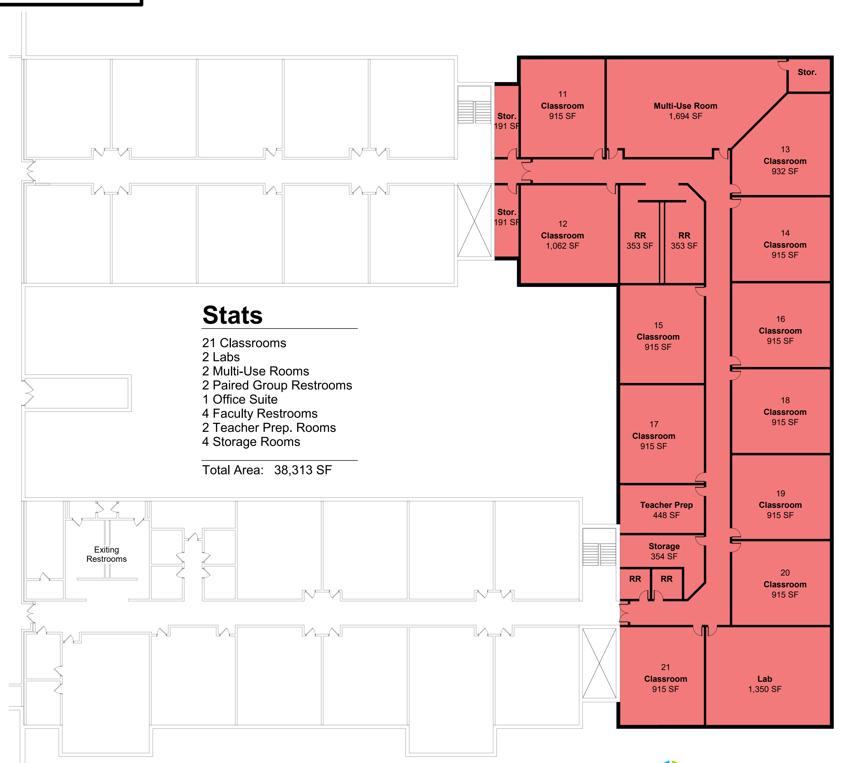
NORTH 3-12 Classroom Addition Second Floor Plan 1/16" = 1'-0" 0 8 16 32
