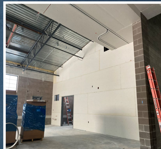
Stage-GWB Hanging & Taping
